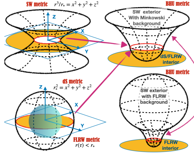
Figure 5. Spatial representation of ds^2 = (1 + 2\Phi)^{-1} dr^2 + r^2 d\theta^2 2D metric embedded in 3D flat space for: deSitter (dS, bottom left, 2\Phi = -r^2/r_s^2 ), FLRW ( r(\tau) < r_s , blue sphere inside dS), Schwarzschild (SW, top left, 2\Phi = -r_s/r ) and two versions of the combined BHU metrics. Yellow region shows the projection coverage in the (x, y) plane. In the top right figure we show a BHU with dS (or FLRW) interior and SW metric exterior joint at the Event Horizon r_s = 2GM = 1/H_\Lambda (red circles). The BHU solution has in general two nested FLRW metrics join by SW metric (bottom right). See Appendix A.
