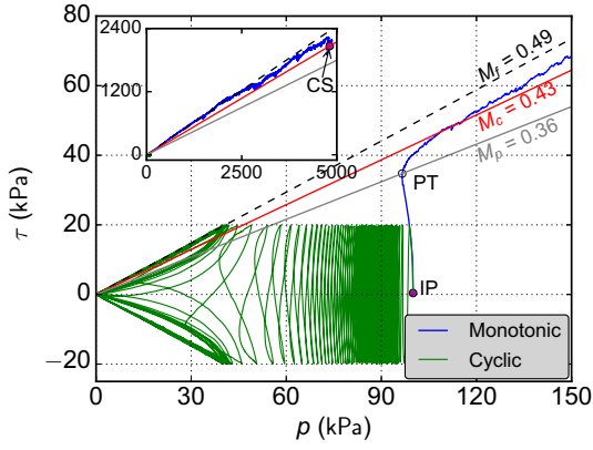
Fig. 4 Comparison of stress paths in constant-volume monotonic and cyclic simple shear tests ( CSR = 0.20 ). IP stands for initial packing, PT for phase transformation, and CS for critical state. The straight lines represent the phase transformation (slope M_p ) and critical state (slope M_c ) based on monotonic test and dilation phase (slope M_f ) based on cyclic test. The inset shows the monotonic shear path at large mean stress values
