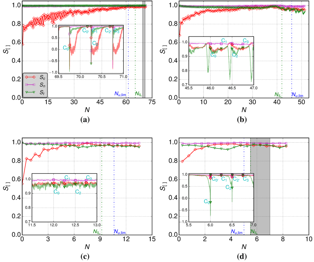
Fig. 18 Evolution of the normalized first joint invariant between fabric tensors and deviatoric stress tensor at C_1 and C_3 of each loading cycle for different shear paths: a 1-D linear; b 2-D linear; c circular; d 8-like. The insets zoom in on a few cycles in the marked window
