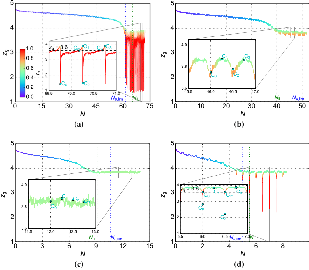
Fig. 12 Evolution of the coordination number z_g under different shear paths: a 1-D linear; b 2-D linear; c circular; d 8-like
