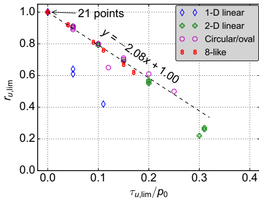
Fig. 9 Relationship between the limit pore pressure ratio r_{u,\text{lim}} and the corresponding shear stress ratio \tau_{u,\text{lim}}/p_0
