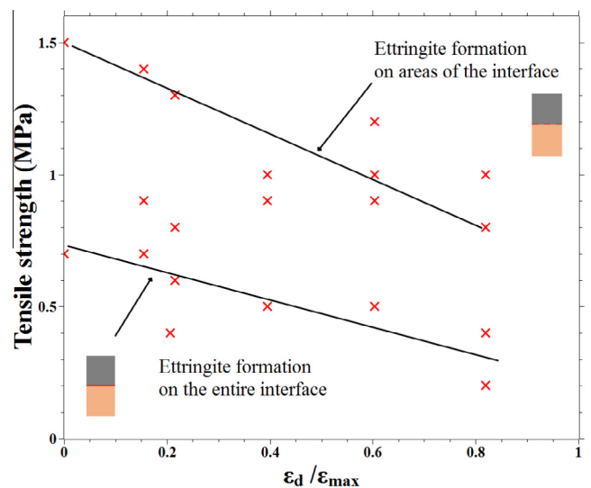
Fig. 21. Evolution of the tensile strength as a function of the degradation ration and assumption of the existence of two zones.
