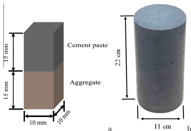
Fig. 1. Geometric configurations and sizes of the samples: a) composite, b) REV sample.
