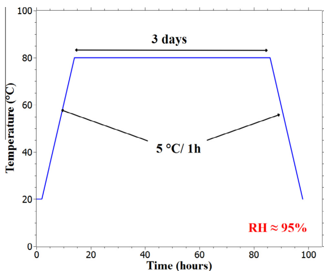
Fig. 2. Hydrothermal treatment applied to the REV sample.
