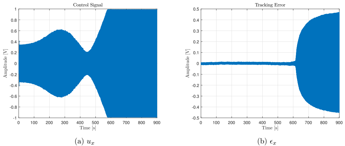
Figure 17: Results of the experiment where the setup is operated in a thermal chamber and where x_{ref}(t) = 0.5 \sin(\omega_{r,x}^{nom} t T_s) .
