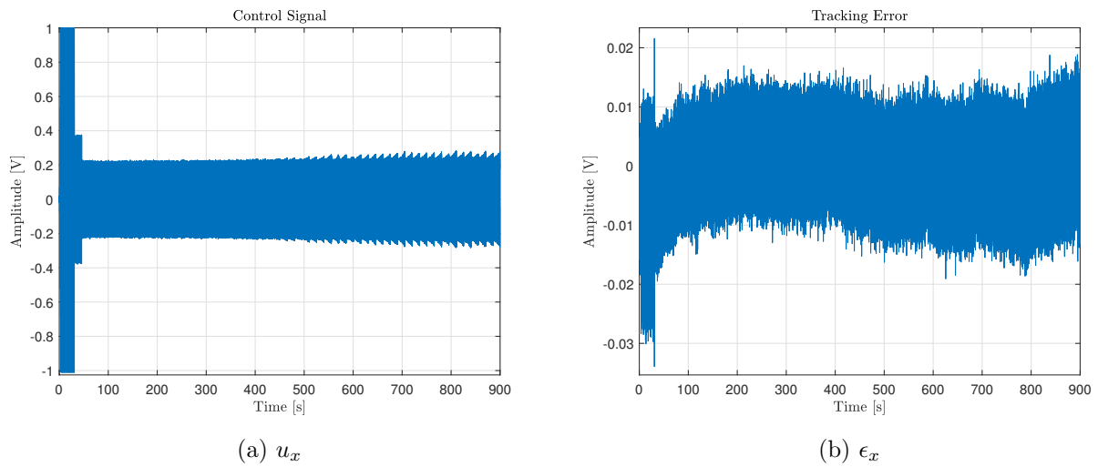
Figure 16: Results of the experiment where the setup is operated in a thermal chamber and where x_{ref} is adapted as shown in Figure 12.
