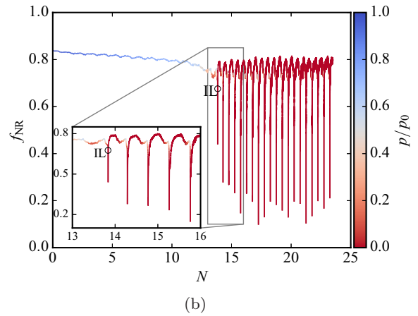
FIG. 4. Evolution of (a) coordination number z_g and (b) non-rattler fraction f_{NR} for simulation T2. The horizontal dashed line z_g \simeq 3.6 refers to the inflection point of z_g .
