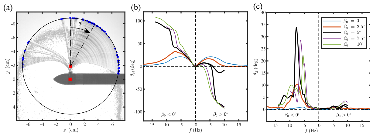
Figure 3. (a) Illustration of the method used to characterise the magnitude of the flapwise blade deformations. (b) Mean deflection \theta_M and (c) amplitude \theta_A of the deformation fluctuation, for all single-bladed rotors tested at constant free-stream velocity.
