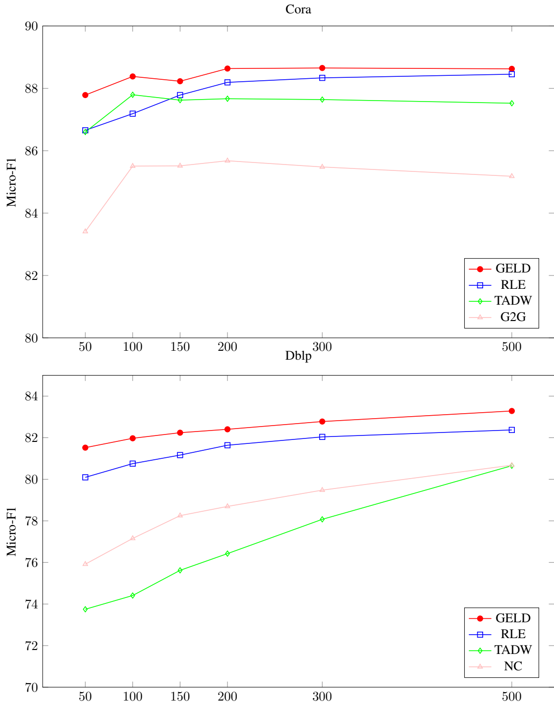
Figure 3: Accuracy with 50% test/train ratio by embedding dimension for the four best methods on the classification task on Dbpl and Cora. NC stands for Naive Combination. GELD performs constantly better than competitors, even in low dimension.
