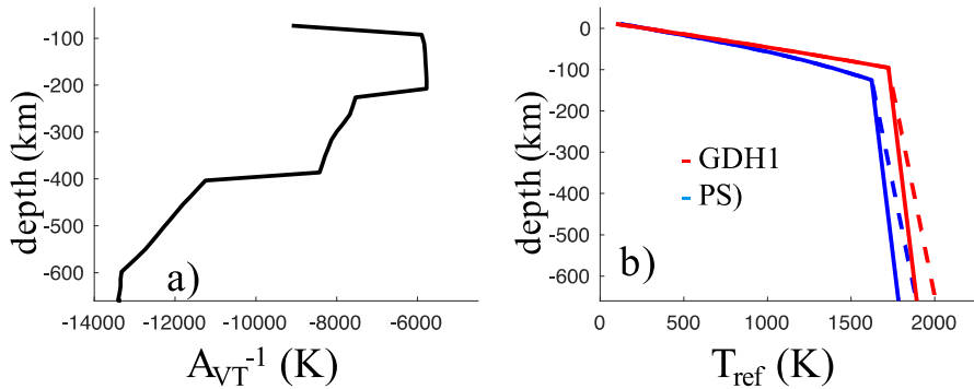
Figure S6: Parameters use to convert the seismic velocity anomalies provided by tomography models, dvs , in temperatures. a) 1/A_{VT} conversion factor obtained by Karato (2008); b) 1D reference temperature profiles. GDH1 (Stein and Stein, 1992) and PS (Parsons et Sclater, 1977) are reported in red and blue respectively. Beneath the lithosphere, we impose a 0.3°/km thermal gradient (dashed blue and red lines) and 0.5°/km (full blue and red lines).
