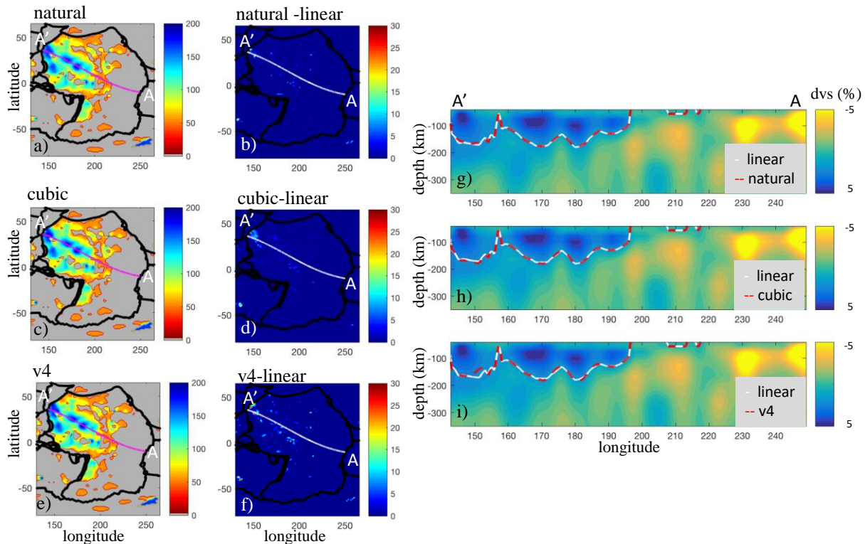
Figure S4: Influence of the interpolation parameters. The color maps displayed in panels a, c and e represent the depth of the LAB obtained with different interpolation methods reported above each panel. The absolute values of the difference between these models and the reference model are displayed in panels b, d and f. Depth cross sections across the tomography model (SEMUCB-WM1) along the AA' profile are reported in panels g, h and i.
