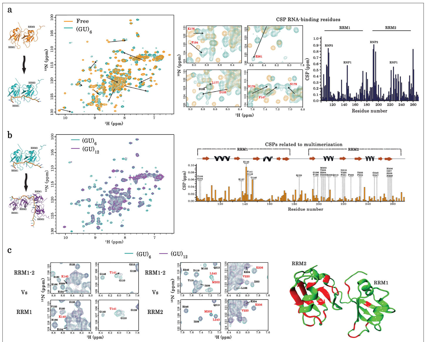
Figure 2. Identification of TDP-43 residues involved in its dimerization on GU-repeats. (a) NMR spectra of free and bound RRM1–2. Left , superimposition of ^1H - ^{15}N SOFAST-HMQC spectra of ^{15}N -labeled RRM1–2 in the free (orange) and (GU)_6 RNA-bound (turquoise) forms. Residues displaying the largest chemical shift perturbations (CSP) are indicated by arrows. Middle , zoom in on NMR spectra (left) showing the CSPs for some residues (highlighted in red) upon (GU)_6 RNA binding. Right , plot of CSPs occurring in RRM1–2 upon (GU)_6 RNA binding. The combined CSPs were calculated as reported (Williamson, 2013) and follow the same trajectories as previously published (Lukavsky et al., 2013) for RRM1–2 bound to AUG12 (PDB 4BS2). (b) NMR spectra of monomeric and dimeric forms of RRM1–2 bound to GU-repeats. Left , superimposition of ^1H - ^{15}N SOFAST-HMQC spectra of ^{15}N -labeled RRM1–2 bound to (GU)_6 (turquoise) or (GU)_{12} (magenta). Right , combined CSPs, observed for monomeric and dimeric couples, plotted and linked to the secondary structures on top. (c) Left , zoom in on NMR spectra (b) showing RRM1–2 residues displaying particular CSPs, resonance disappearing, or peak broadening (in red) as compared to respective residues in RRM1 or RRM2 fragments. Right , all affected residues upon RRM1–2 dimerization are highlighted in red using molecular modelling approaches on RRM1–2 free fragment (see methods). Based on the above comparative NMR study, 28 residues were selected as candidates for mutagenesis approach combined to a detailed cellular and biochemical investigation.
