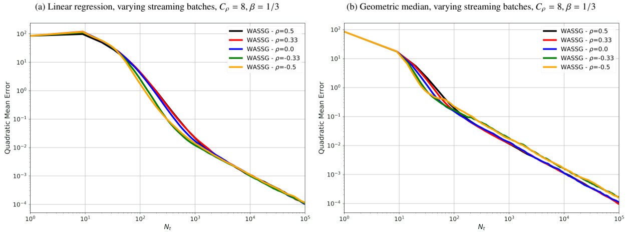
Figure 3: WASSG for various data streams n_t = C_\rho t^\rho . See Section 6 for details.
