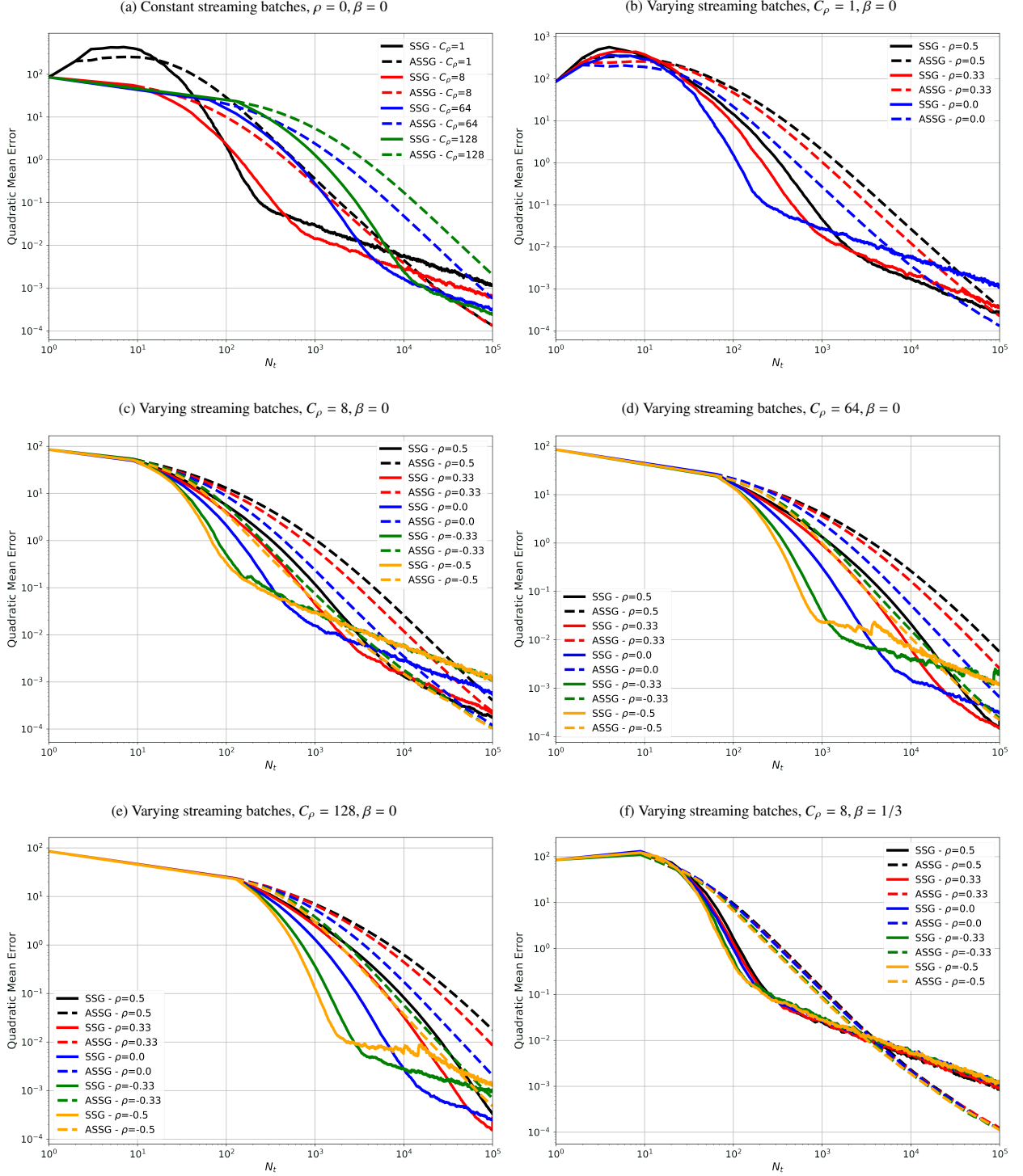
Figure 1: Linear regression for various data streams n_t = C_\rho t^\rho . See Section 5.1 for details.
