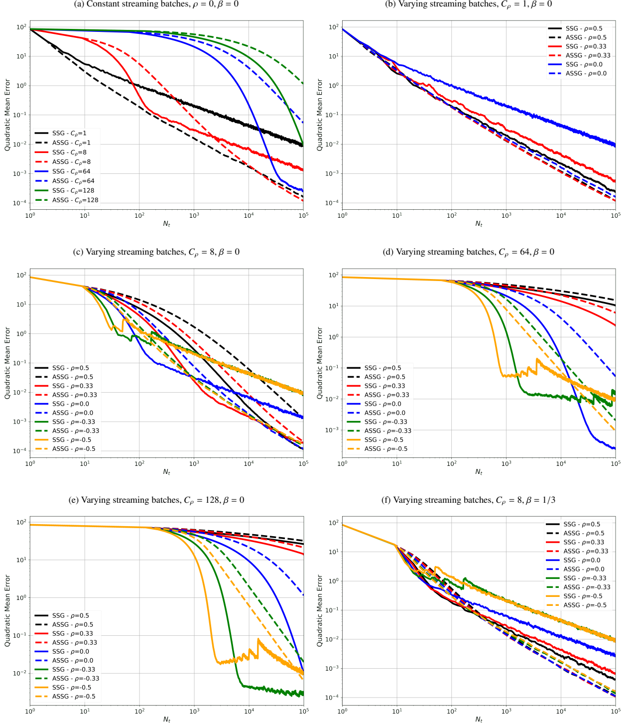
Figure 2: Geometric median for various data streams n_t = C_\rho t^\rho . See Section 5.2 for details.
