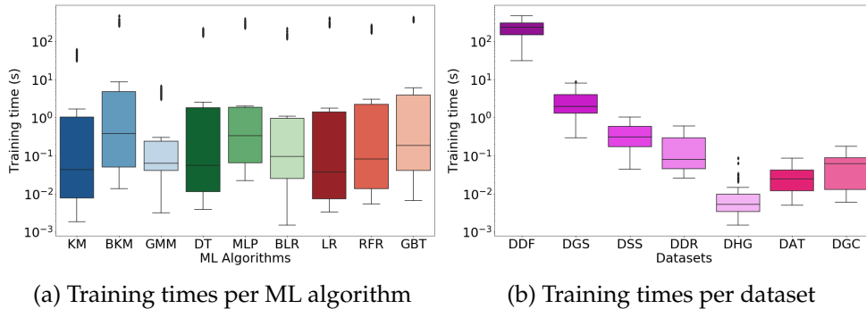
Figure 2: Statistical analysis of training times for different ML algorithms and datasets
