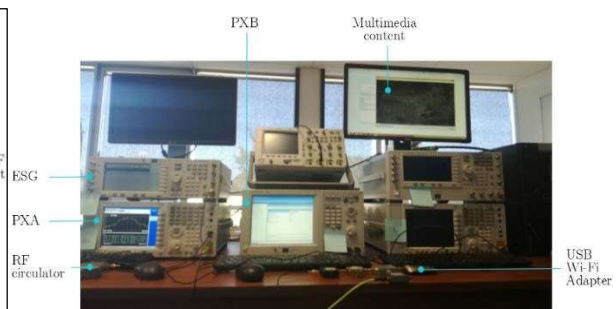
Fig. 4 Set up in the lab with PXB channel emulator
