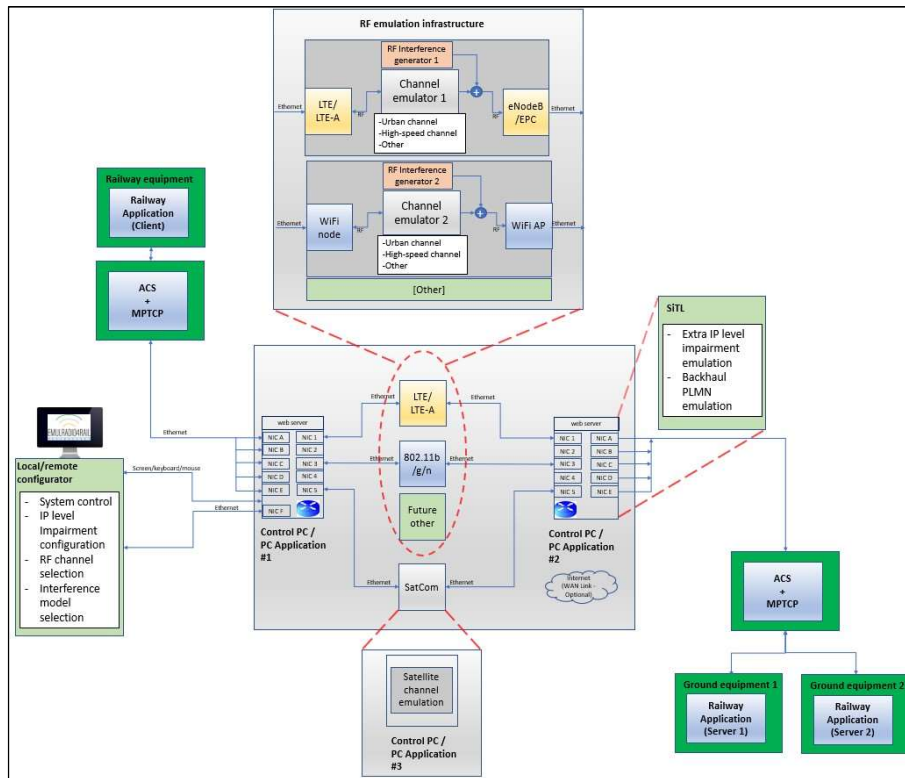
Fig. 1 General high level architecture of the EMULRADIO4RAIL platform
