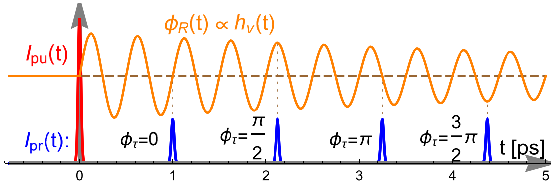
Figure 7. Role of interference between the incident probe pulse spectrum and scattering to spectral sidebands. We consider impulsive excitation by the pump pulse (red), followed by the probe pulse (blue) delayed by four different times so that the vibrational phase, \phi_\tau = \{0, 1/2, 1, 3/2\} \pi at our example probe pulse time delays. These time-delays are chosen to illustrate the interference process that produces a varying shift in the probe pulse power spectral density center of mass (COM) as a function of probe pulse delay \tau that are shown in figure 8.
