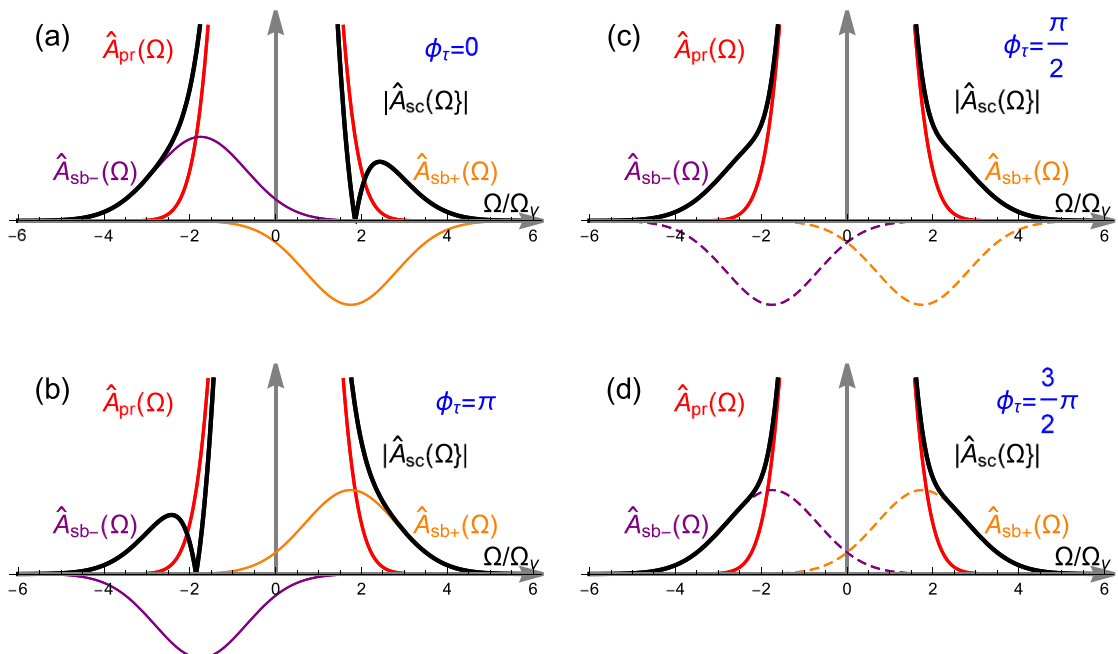
Figure 8. Examples of spectral sideband interference that depend on the vibrational phase \phi_\tau = \Omega_v \tau . (a), (b) For \text{mod}_2 \pi [\phi_\tau] = \{0, \pi\} , the scattered sidebands are purely real and directly interfere with incident probe pulse spectrum. (a) When \text{mod}_2 \pi [\phi_\tau] = 0 , the positive sideband is negative valued, whereas the negative sideband is positive valued—producing a spectral center of mass shift to positive values: \langle \Omega \rangle > 0 . (b) At \text{mod}_2 \pi [\phi_\tau] = \pi , the signs of the sidebands reverse, leading to \langle \Omega \rangle < 0 . (c), (d) By contrast, at time delays that produce \text{mod}_2 \pi [\phi_\tau] = \{\pi/2, 3\pi/2\} , the sidebands are completely imaginary, preventing interference so that all three spectral distributions add in quadrature—producing symmetric spectral broadening and \langle \Omega \rangle = 0 . All other time delays drive spectral scattered sidebands that are complex, leading to an intermediate shift in the spectral center of mass.
