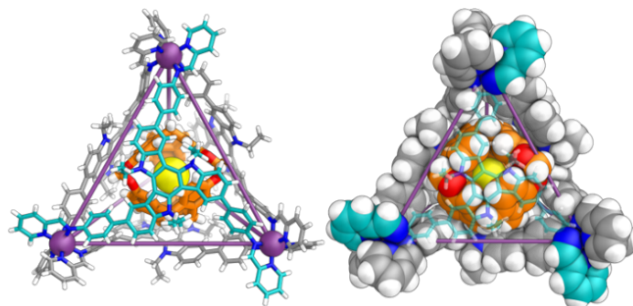
FIGURE 38: Crystal structure of [Cs + @ PP-54 ] c Δ 4 -Fe II 4 L 4 illustrating the [Cs + @ PP-54 ] c Δ 4 -Fe II 4 L 4 enantiomer. The bound Cs + , PP-54 and the front triazatruxene face are colored yellow, orange and cyan, respectively. Disorder, unbound counterions, and solvent of crystallization are omitted for clarity and only one of the two crystallographically independent complexes is shown. Adapted with permission from ref. 117. (2019) American Chemical Society.
