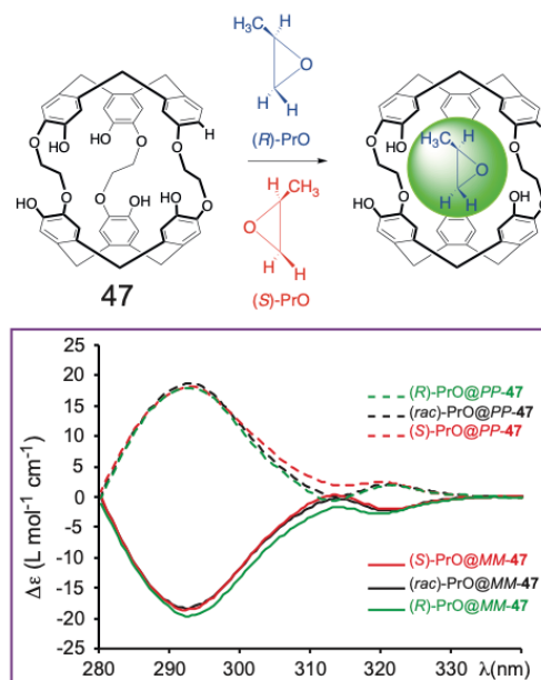
FIGURE 28: Left) Preferential encapsulation of (R) -PrO by cryptophane PP - 47 . Right) ECD spectra recorded at 275 K of diastereomers (R) -PrO@ MM - 47 , (S) -PrO@ MM - 47 and (rac) -PrO@ MM - 47 , (R) -PrO@ PP - 47 , (S) -PrO@ PP - 47 and (rac) -PrO@ PP - 47 . Only the Cotton bands corresponding to the 1 L b transition are shown. Adapted with permission from ref. 91. (2011) American Chemical Society.
