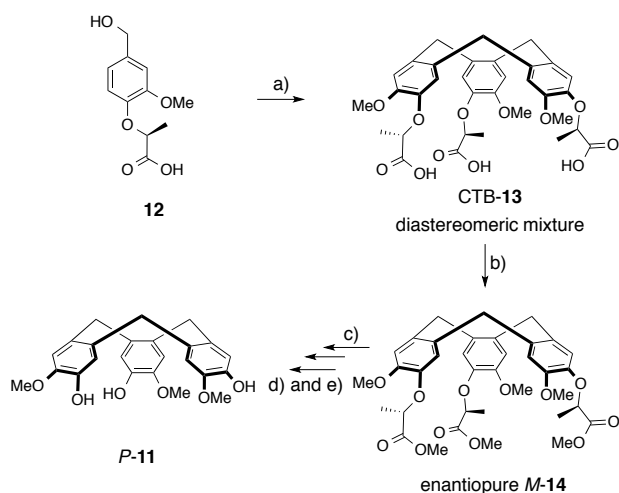
FIGURE 5: Synthesis of enantiopure CTG 11 derivative from enantiopure vanillic alcohol derivative 12 . a) \text{HClO}_4 , 65%, b) \text{CH}_2\text{N}_2 , 32% c) \text{LiAlH}_4 , THF, 99% d) \text{MsCl} , pyridine, 87% then \text{MgI}_2 , ether/ \text{CH}_2\text{Cl}_2 69% e) \text{Zn} , \text{CH}_3\text{CO}_2\text{H} , 91%.
