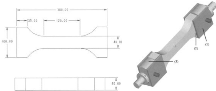
Fig. 1. a Direct tensile specimen – b Grip system
