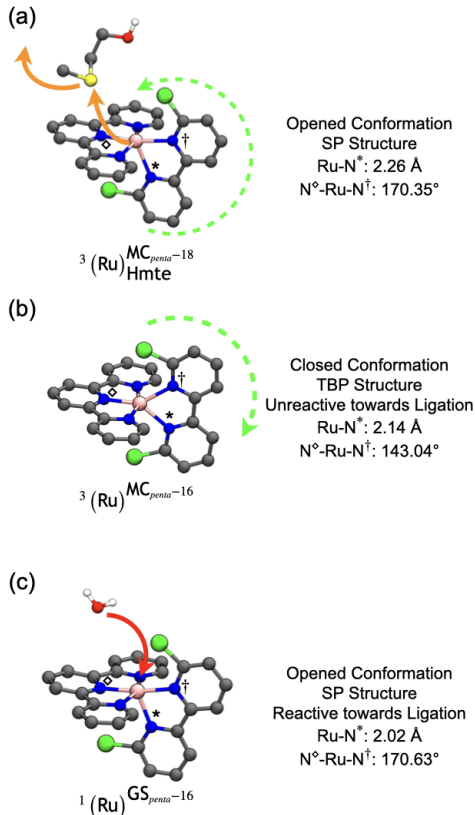
Figure 2: Schematic representation of the intramolecular rearrangements occurring in the key species involved in ligand exchange. (a) Diffusion of the Hmte ligand and closing of the dcbpy ligand ( Step 1 ). (b) Opening of the dcbpy ligand (end of Step 2 ) and (c) binding of a water molecule ( Step 3 ). Distances and angles are from the static DFT-optimized minima.
