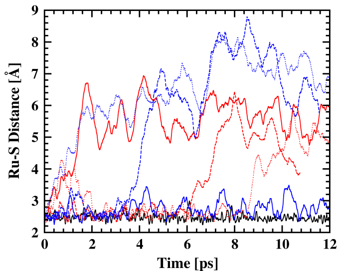
Figure 1: Time evolution of Ru-S distance during AIMD simulations consisting in 103 water molecules and one ^1(\text{Ru})_{\text{Hmte}}^{\text{GS}} (black plain line ; canonical simulation) or one ^3(\text{Ru})_{\text{Hmte}} (blue and red lines ; microcanonical simulations) complex. In the former case, the simulation is 75 ps long although only the first 12 ps are displayed. The average Ru-S distance over the whole simulation is 2.45 Å, which is slightly larger than the value obtained from static geometry optimization (2.40 Å; see Table S1 and Figure S1), and the standard deviation is 0.08 Å. When switching to the lowest energy triplet state, fluctuations of the Ru-S distance increase significantly and the Hmte ligand can move further away from the complex as fast as \sim 1 ps. Only one simulation does not lead to dissociation before 12 ps (blue plain line).
