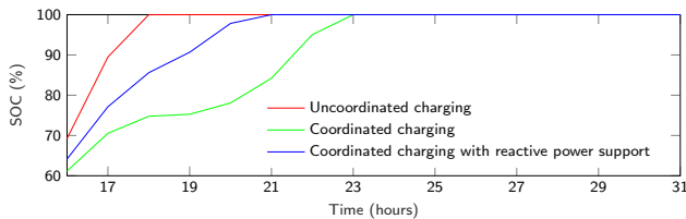
Fig. 4. Average SOC across the EVs population.
