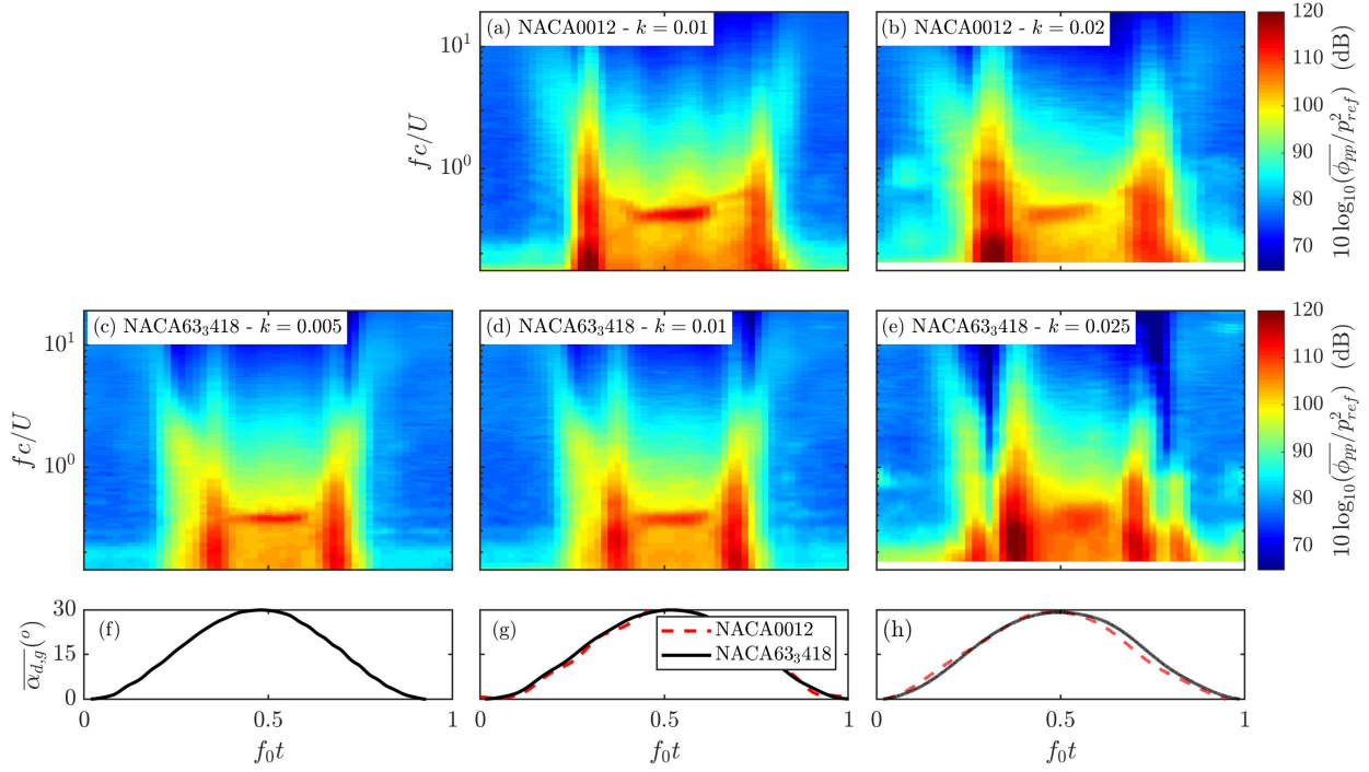
Fig. 8 Phase-averaged spectrograms of surface pressure at x/c = 0.92 on the suction side for \alpha_{d,g} = 15^\circ + 15^\circ \sin(2\pi f_0 t) for (a-b) the NACA0012 airfoil and (c-d-e) the NACA63418 airfoil, and (f-g-h) phase-averaged angle of attack. The overbar denotes phase-averaging.
