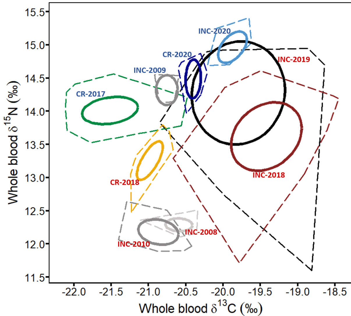
Figure 4: Whole blood \delta^{13}\text{C} and \delta^{15}\text{N} values of common diving petrels ( P. urinatrix ) from Kanowna Island in incubation (INC: red, 2018, n = 23 ; black, 2019, n = 20 ; light blue, 2020, n = 9 ) and chick-rearing (CR: green, 2017, n = 51 ; yellow, 2018, n = 16 ; dark blue, 2020, n = 15 ). Incubation 2008-2010 (grey) are whole blood \delta^{13}\text{C} and \delta^{15}\text{N} values of common diving petrels in incubation from Kanowna Island obtained from Fromant et al., 2020 (2008, n = 10 ; 2009, n = 4 ; 2010, n = 15 ). Full lines correspond to the 40% ellipse and dashed lines 100% total convex hull. The blue and red writing represent cold and warm years, respectively (see Figure 1).
