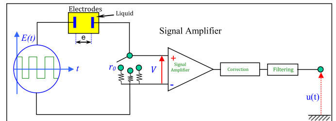
Fig. 4. Simplified sketch of the conductimetry measurement device.
