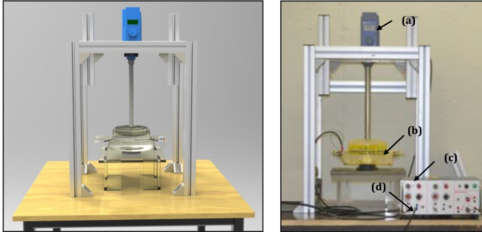
Fig. 1. 3D conception (left) versus real experimental (right) setup: (a) Electrical motor; (b) Film recipient; (c) Conductimetric device; (d) Output to acquisition system.
