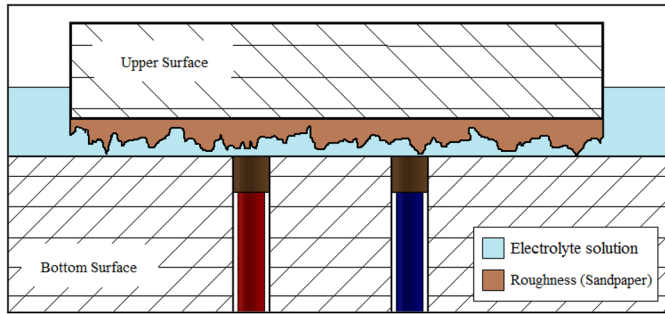
Fig. 7. Schematic representation of the experimental measuring principle.
