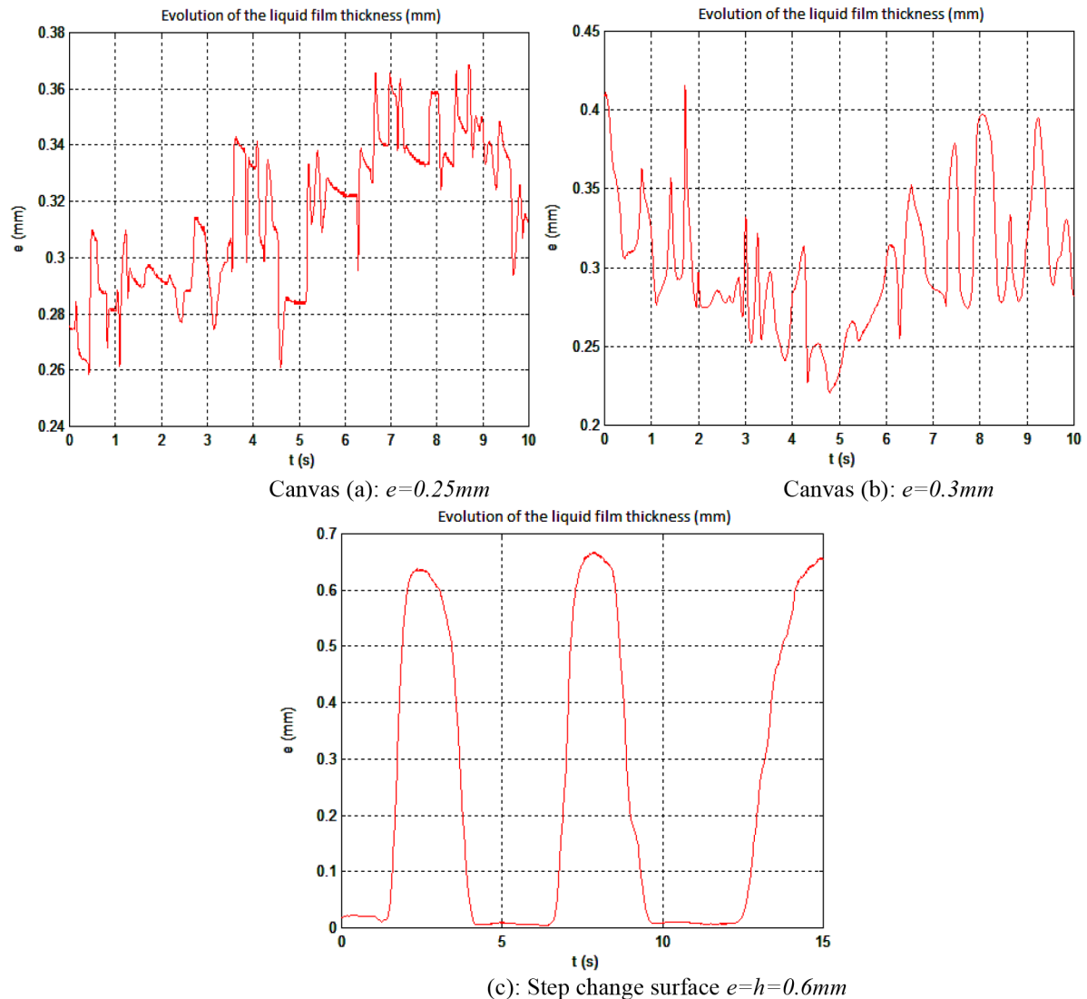
Fig. 11. Conductimetric probes' responses of the specific used surfaces.
