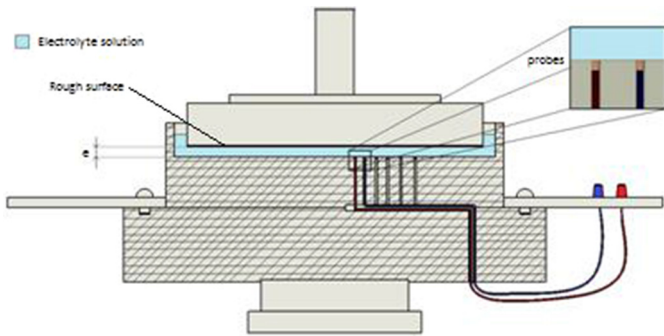
Fig. 3. Measurement test-section of liquid film thickness “e”.
