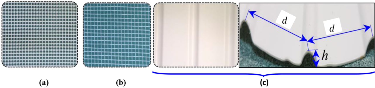
Fig. 10. Specific used surfaces: (a) Plastic canvas ( e = 0.25 mm); (b) Plastic canvas ( e = 0.3 mm); (c) Plastic canvas ( e = h = 0.6 mm).
