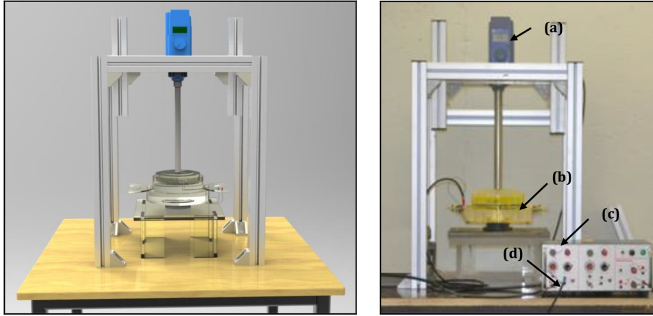
Fig. 1. 3D conception (left) versus real experimental (right) setup: (a) Electrical motor; (b) Film recipient; (c) Conductimetric device; (d) Output to acquisition system.
