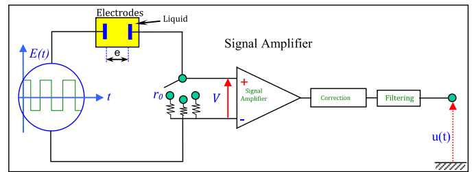
Fig. 4. Simplified sketch of the conductimetry measurement device.
