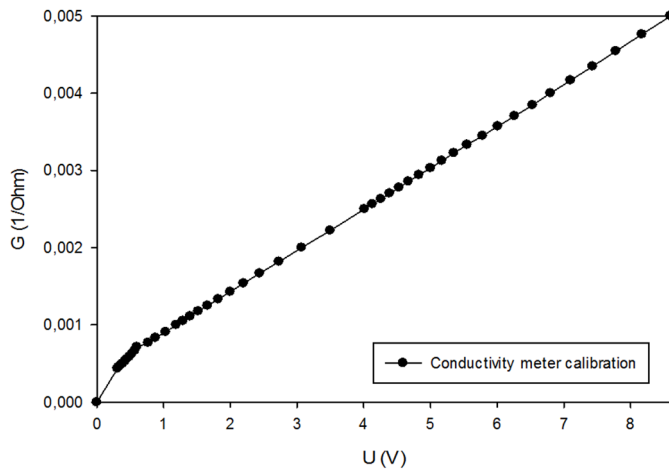
Fig. 5. Calibration of the conductimetric system using passive resistances at f = 50 kHz.
