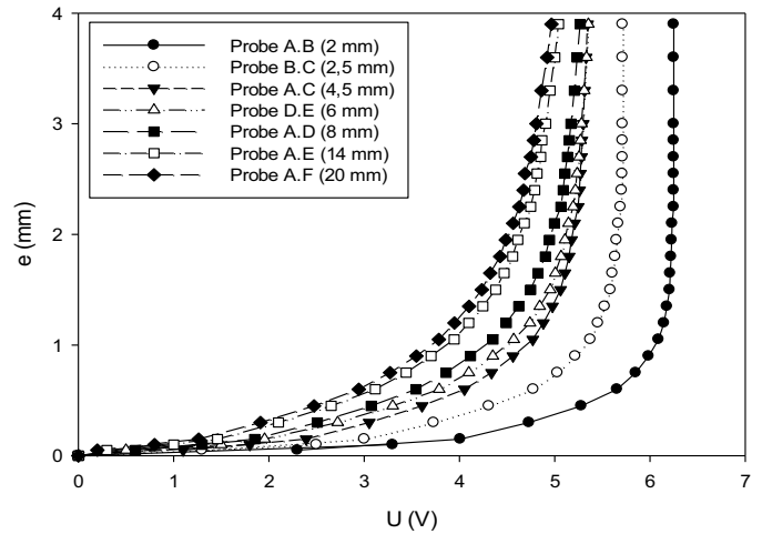
Fig. 6. Calibration curves for the different conductimetric probes.
