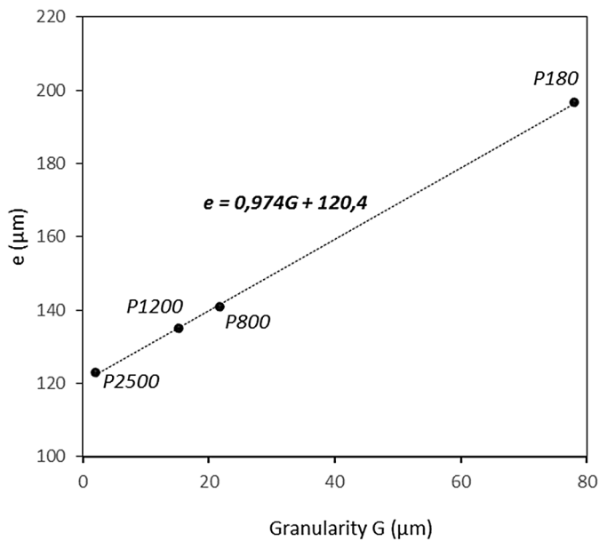
Fig. 8. Liquid film thickness obtained for different rough surfaces during static trial.
