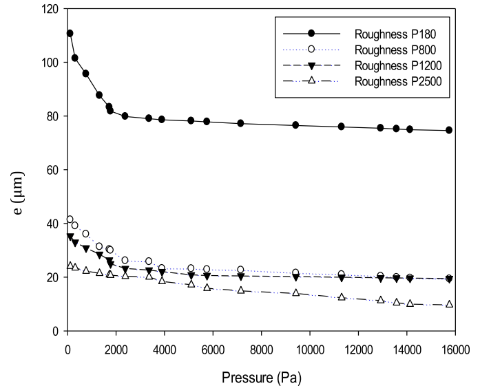
Fig. 9. Effect of pressure load on the liquid film thickness.
