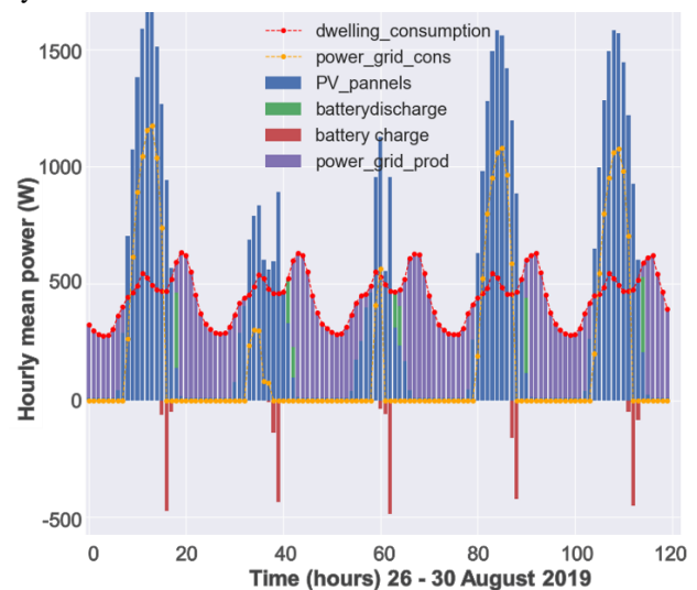
Figure 3: Dwelling energy flows diagram from OMEGAAlpes
