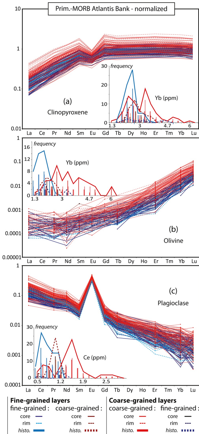
Figure 8. Rare earth element (REE) normalized to the average of the most primitive mid-ocean ridge basalt sampled on the Atlantis Bank section of the SWIR (from Coogan et al., 2004; Table S5) concentration diagrams for (a) Cpx, (b) Ol, and (c) Pl from section 65R5. Solid and dashed lines indicate crystal cores and rims, respectively. Histograms indicate the compositional distribution of the most abundant REE analyzed in Pl and Ol, and that of the most fractionated REE in Cpx. The frequencies represent the total number of analyses for each lithology, which are lower for the fine-grained compared to the coarse-grained layers (by 40 for Pl and Cpx, and 30 for Ol).
