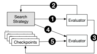
Fig. 6: Software Architecture of Our Implementation
