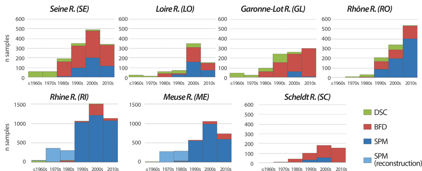
Fig. 2. Distribution of the number of samples with metallic element data according to matrix types, rivers and time. BFD = bed and flood deposits, DSC = dated sediment cores, SPM = suspended particulate matter.
