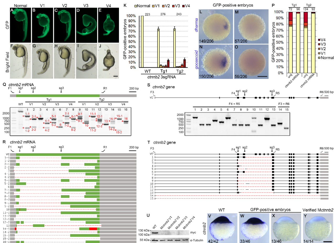
96 Figure 4. Generation of ctnnb2 maternal mutants and large deletions by transgenic 97 expression of multiple Cas9 RNPs. (A-J) Phenotypes of GFP-positive embryos simultaneously 98 expressing three sgRNAs targeting ctnnb2 . (K) Statistical analysis of ventralized phenotypes in 99 GFP-positive offspring derived from two mutation-carrying Tg( zpc:zcas9 ) F0 fish. Numbers 00 designate total embryos analyzed. Error bars indicate standard deviations (SD) from three 01 independent spawnings. (L-O) Absence of dharma and goosecooid expression in GFP-positive 02 Mctnnb2 embryos. Scale bars: 250 \mu m. (P) The ventralized phenotype in GFP-positive Mctnnb2 03 embryos can be rescued by overexpression of the wild-type ctnnb2-myc mRNA. Numbers on top 04 of each column represent total embryos scored. Tg1 and Tg2 are two independent mutation- 05 carrying F0 fish. (Q) RT-PCR analysis of the CDS region from 16 Mctnnb2 mutant embryos. 06 Wild-type (WT) embryos served as a control. Deletion alleles were present in all mutant embryos 07 tested. V1 to V4 indicate the degrees of ventralized phenotypes, as shown in (A-J) . Asterisks and 08 numbers designate PCR products subjected to Sanger sequencing. F1 and R1 are primers used to 09 amplify the CDS region of ctnnb2 transcripts. The positions of the three sgRNA targeting sites are 10 indicated as sg1, sg2, and sg3. Grey boxes indicate UTRs; the green box represents the CDS 11 region; dashed lines represent deletions; red boxes indicate insertions. (R) Sequencing results of
