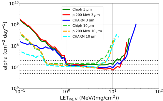
Fig. 6. Alpha factor as a function of the volume equivalent LET for the SEL SV with 3 \mu\text{m} and 10 \mu\text{m} thicknesses for the various facilities.
