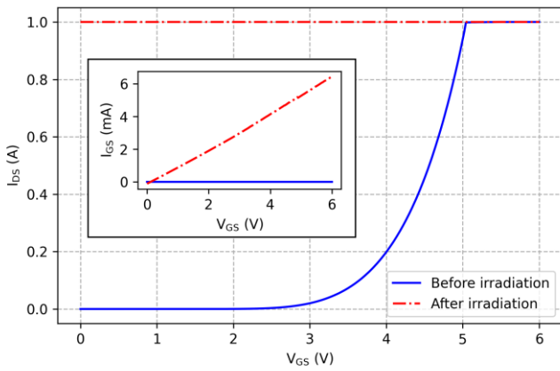
Fig. 3. I_{DS}V_{GS} and I_{GS}V_{GS} characteristics of the failed device before and after irradiation. Device was irradiated at V_{DS} = 675 V and V_{GS} = 0 V Both drain-source and gate failures can be observed after irradiation induced failure. I_{DS} reaches the compliance limit of the measurement unit at 1 A.
