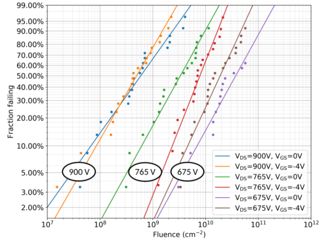
Fig. 2. Weibull plots for different bias voltage configurations during irradiation. Fits are performed with MLE method.
