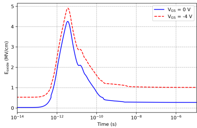
Fig. 10. Simulated time evolution of electric field in the gate oxide layer during the ion impact for V_{DS} = 675 V bias configuration. The applied reverse gate bias results in higher electric field in the oxide during the charge deposition in the device for an ion impact in the neck region.
