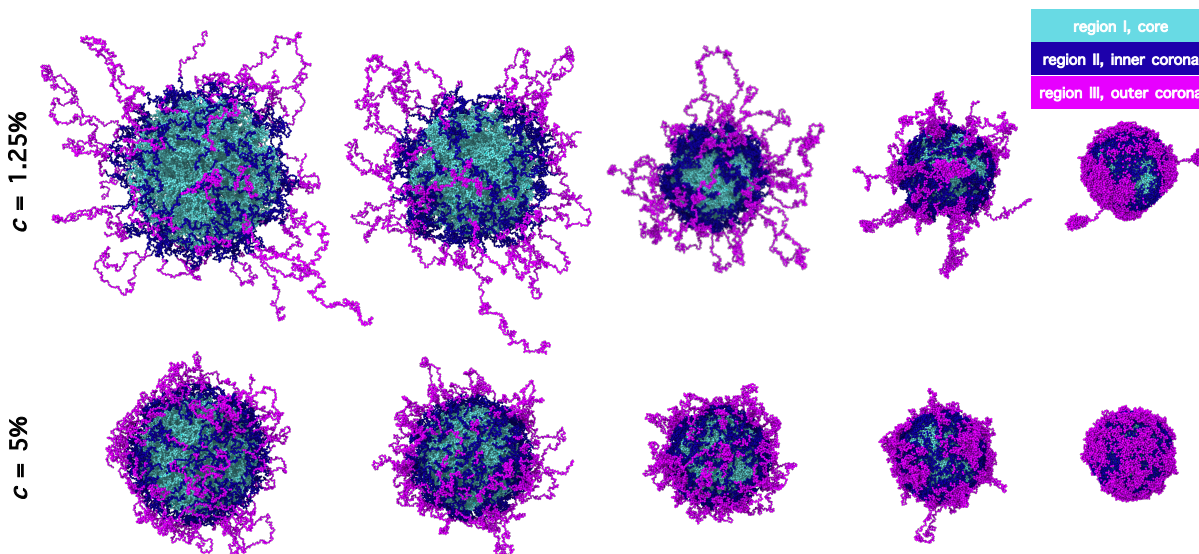
FIG. S4: Snapshots of surface charged microgels across the VPT illustrating the local swelling. Simulation snapshots for a surface-charged microgel ( f = 3.2\% ) for different values of the swelling parameter \alpha from the swollen to the collapsed state. From left to right, for c = 1.25\% , \alpha = 0.0, 0.48, 0.80, 0.90, 1.20 , while for c = 5\% , \alpha = 0.0, 0.48, 0.74, 0.90, 1.20 . Monomers are colored according to the region they belong to: cyan indicate the core region (defined as 65% of most inner particles), blue the inner corona region (consisting of 20% of monomers nearest to the core beads) and purple the outer corona region (comprising the 15% most exterior beads).
