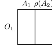
Fig. 4: Aggregation
