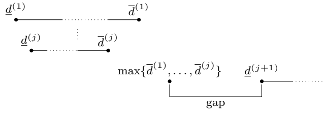
Fig. 4 Case where \cup_{i=1}^I [\underline{d}^i, \bar{d}^i] is not an interval
