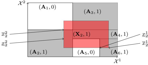
Fig. 5 Example of determining the single effect
