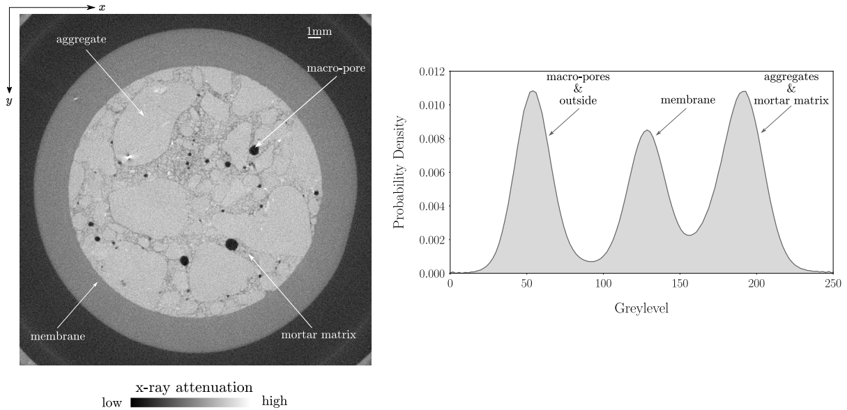
Figure 2: Mid-height horizontal slice and greylevel histogram of the reconstructed 3D volume of the TX10-01 test
