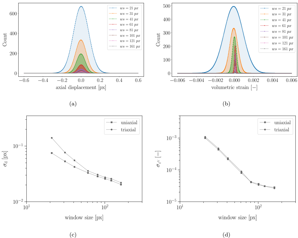
Figure 6: Estimation of DVC measurement uncertainties for uniaxial (PMAA cell) and triaxial (aluminium cell) tests. (Top): Histograms of measured axial displacement (a) and volumetric strain (b) for a range of window sizes for the uniaxial tests. (Bottom): Evolution of the standard deviation of the displacement magnitude (c) and the volumetric strain (d) as a function of the correlation window size for both types of tests
