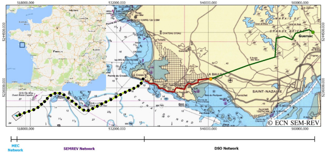
Figure 1. The SEM-REV open sea test site is located in western France, near Le Croisic. The physical installation of the 24 km export cable studied in this paper follows the dotted path. It connects the SEM-REV offshore hub to an onshore substation and finally to the local network belonging to French DSO Enedis (red and dark green paths). Figure modified, courtesy of École Centrale de Nantes [19].
