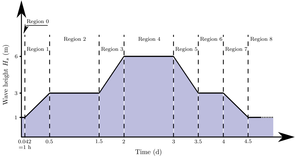
Figure 5. Sequence of sea-states that has been used for all simulation cases (see Table 1). Note that it is a completely fictitious sequence but based on plausible durations and transitions between each sea-states based on Fig. E2 and E3 of [41].
