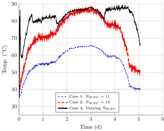
Figure 6. Cores temperature calculated for Case 1 to Case 3, with respectively 11, 13 and 13 to 15 WECs. Compared to Case 1 and 2, Case 3 shows cores temperature that remain closer to T_{max} = 90 °C over time.
