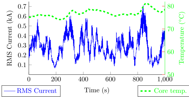
Figure 2. Example of a RMS current profile generated by a WEC farm composed of 20 WECs considering a H_s = 6 m and T_p = 9 s sea-state. One can see the high current fluctuations while the temperature of the core of a phase remains almost constant.
