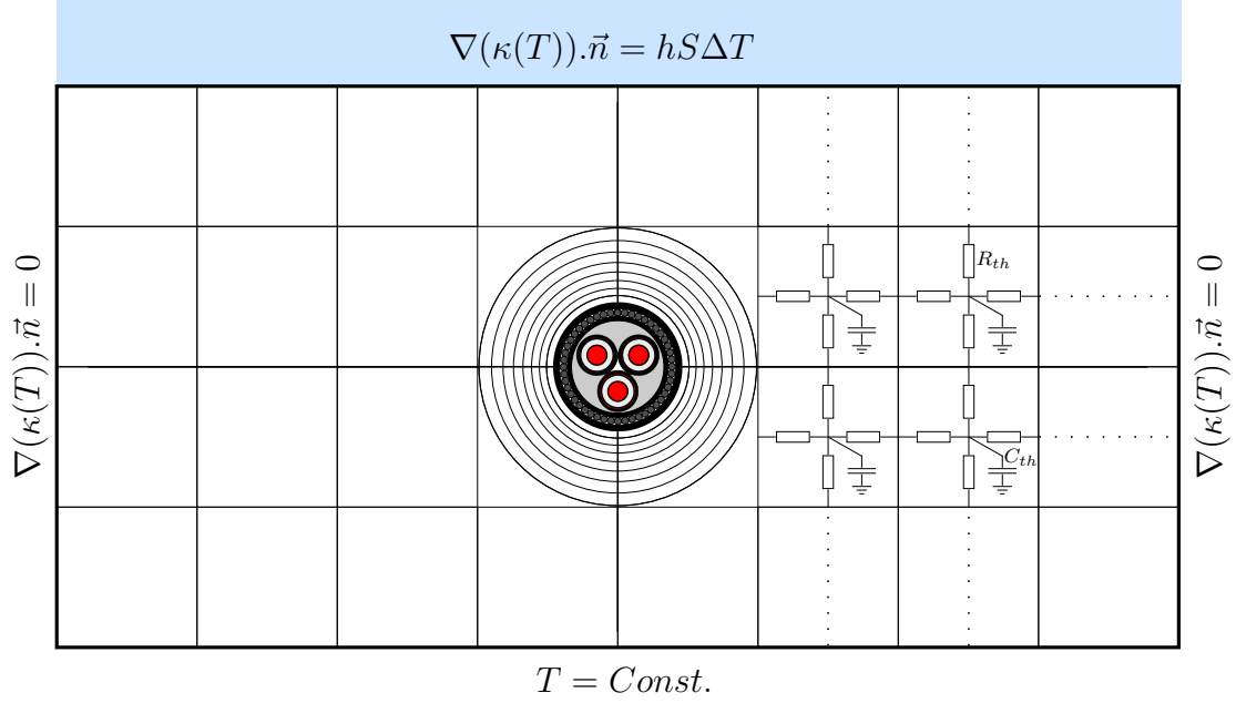
Figure 4. Discretization of cable and of its direct environment as implemented under Matlab ® where we used elements of different sizes (not to scale). The sea surface is not discretized in electro-thermal elements and we only considered a boundary condition for the heat transfer as described in eq. (2). One can see the thermal equivalent electric circuits composed of non-linear resistors R_{th} and capacitors C_{th} that are used to discretized the geometry.
