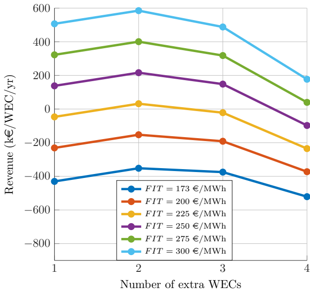
Figure 7. An optimal number of 2 additional WECs maximizes the benefits per WEC, which brings the number of WEC to 13. One can also remark that the economical profitability is not guaranteed for the lowest FITs.
