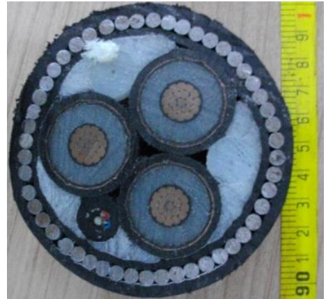
Figure 3. Cross section picture of the export cable considered for our case studies. The cable is currently installed in the SEM-REV test site located off Le Croisic (see Fig. 1), France and is managed by École Centrale de Nantes [19].
