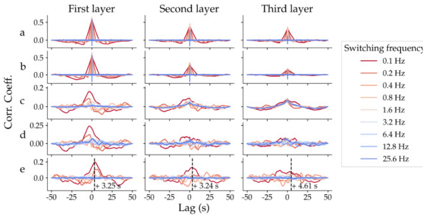
Figure 7: (a) «without astrocyte» mean correlation coefficient of the neuronal's firing rate (excitatory and inhibitory) with the input signal pattern. (b) «with astrocyte» mean correlation coefficient of the neuronal's firing rate (excitatory and inhibitory) with the input signal pattern. (c) neuronal's firing rate (excitatory and inhibitory) mean correlation coefficient with the astrocytic activity. (d) AMPAR density expression's mean correlation coefficient with the astrocytic activity. (e) Astrocytic activity (see section 2.9) mean correlation coefficient with the input signal pattern. The dashed line indicates the lag of higher correlation coefficients average.
