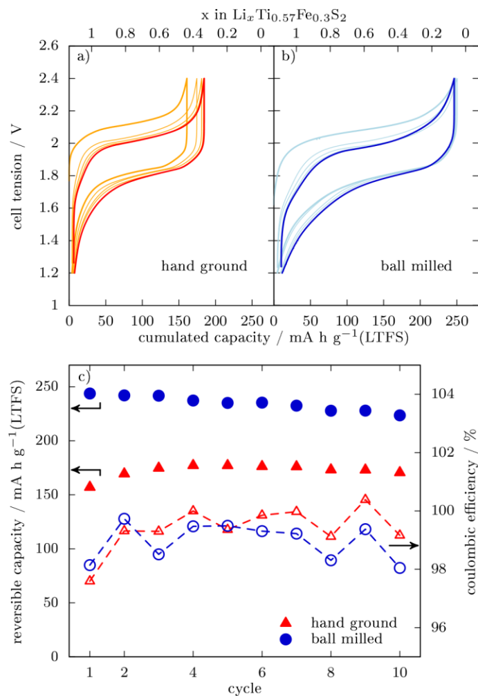
Figure 4: voltage profile of LTFS vs. \text{Li}_{0.5}\text{In} anode for hand ground composite (a) and ball-milled composite (b) at C/25 ; reversible capacity and coulombic efficiency of both cells (c).
