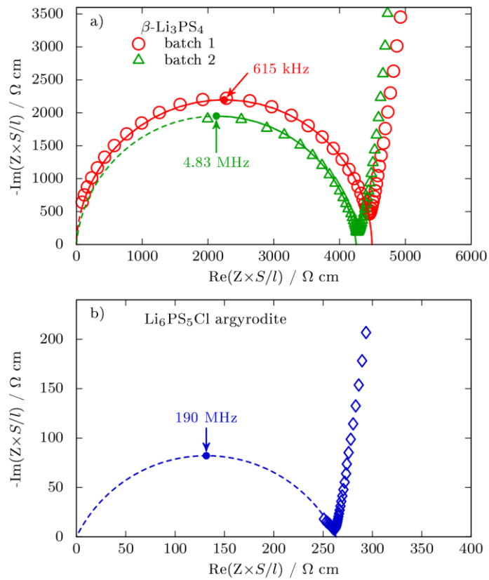
Figure 3: complex resistivity of solid electrolyte pellets: a) \beta\text{-Li}_3\text{PS}_4 and b) \text{Li}_6\text{PS}_5\text{Cl} . The high frequency response is fitted with the impedance of a parallel R-CPE circuit (solid lines) and extrapolated until Z = 0 at infinite frequency (dashed line).
