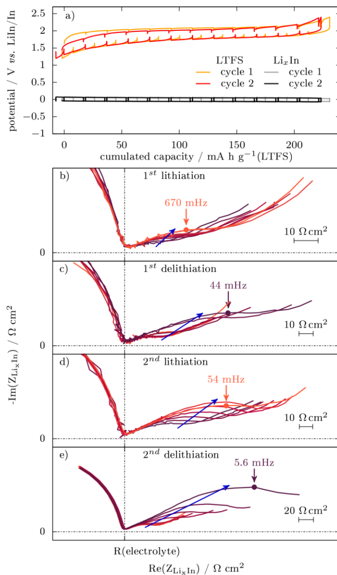
Figure 9: galvanostatic voltage profiles of LTFS WE and Li 0.5 In CE under 1 t cm -2 (a) for the first 2 cycles; impedance of the Li-In alloy CE (b-e) for each charge and discharge sequence. Blue arrows indicate the evolution of the impedance at each sequence.
