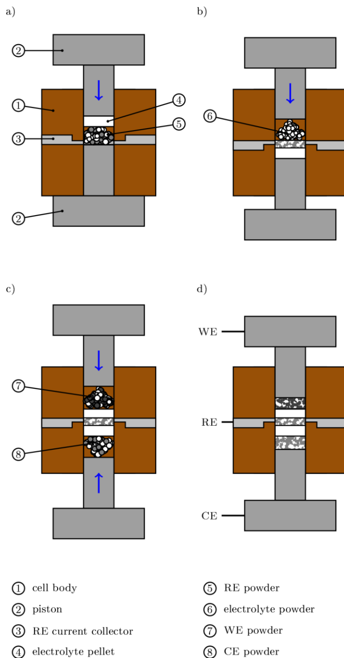
Figure 2: assembly procedure of the 3 electrodes all solid state cell: a) assembly of the reference layer with a solid electrolyte pellet; b) addition of a 2nd electrolyte layer; c) addition of working and counter electrodes; d) cell ready to cycle. Blue arrows indicate the displacement of mobile pistons w./ respect to the cell body at each step.
