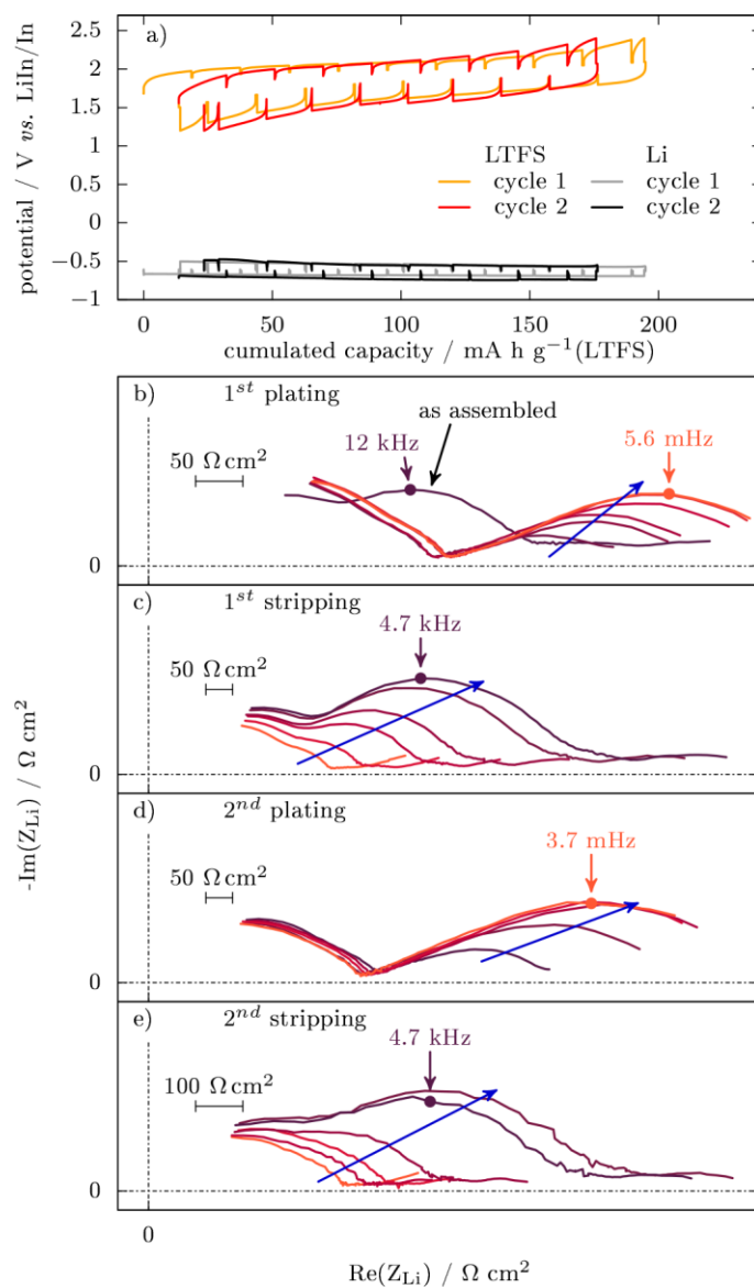
Figure 10: galvanostatic voltage profiles of LTFS WE and Li CE (a) under 45 kg cm -2 for the first 2 cycles; impedance of the Li metal CE (b-e) for each charge and discharge sequence. Blue arrows indicate the evolution of the impedance at each sequence.
