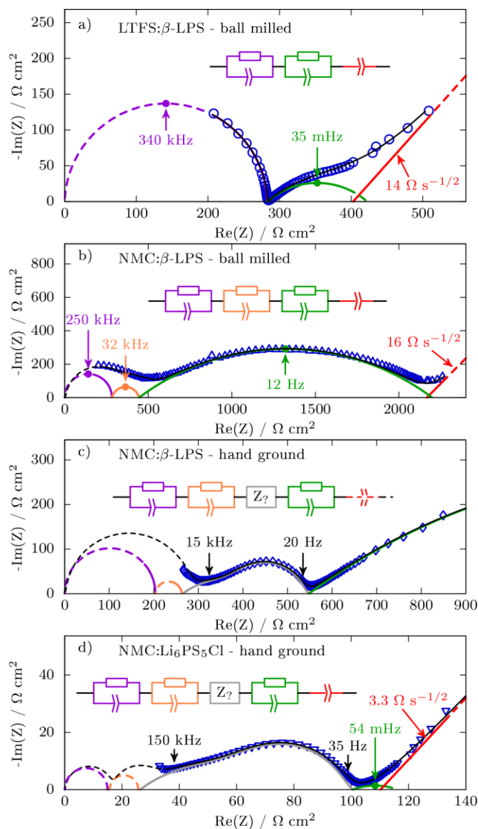
Figure 6: impedance of the various WE composites recorded at the middle of 2 nd reduction: a) ball-milled LTFS:β-LPS; b) ball-milled NMC622:β-LPS; c) hand ground NMC622:β-LPS; d) hand ground NMC622:Li 6 PS 5 Cl. A black line indicates the fit of the spectra with a series of parallel R-CPE elements depicted in each subfigure. The impedances of their constitutive elements are plotted with their respective colour. In c) and d) Z ? is a series of two R-CPE elements.
