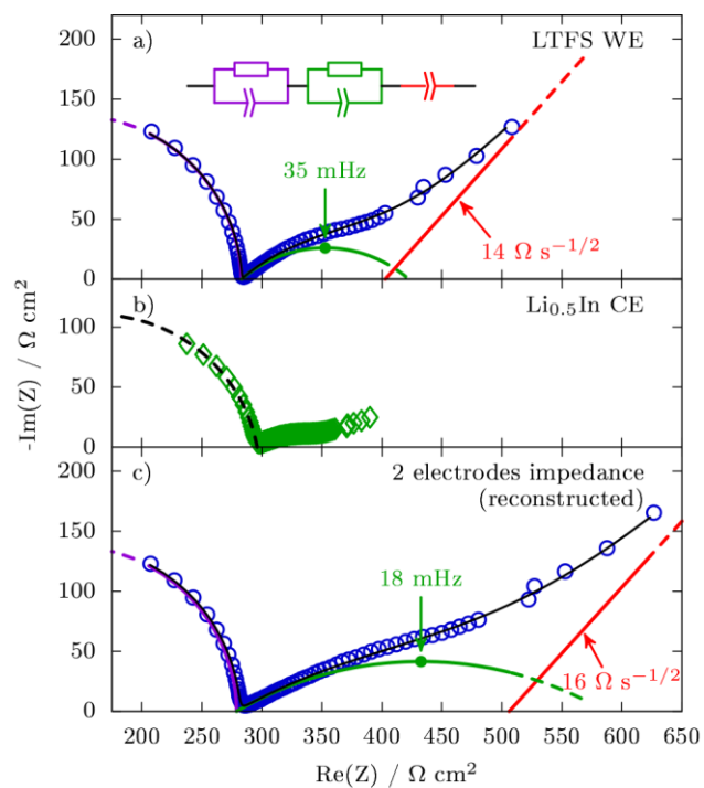
Figure 7: a) impedance of partially lithiated LTFS recorded in the middle of 2nd discharge (open symbols); b) impedance of the \text{Li}_{0.5}\text{In} counter electrode simultaneously recorded; c) impedance of a 2 electrodes LTFS: \text{Li}_{0.5}\text{In} cell as reconstructed from the spectra in a) and b). The spectra in a) and c) are fitted using the equivalent circuit displayed in a) (solid lines).
