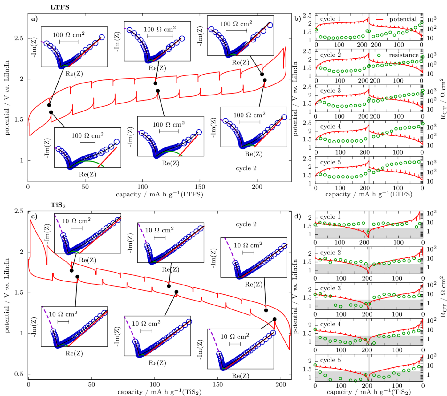
Figure 8: 2nd cycle and variations of R_{CT} during cycling for LTFS (a) and b), respectively) and TiS_2 (c and d). Insets in a) and c) report the impedance spectra of LTFS and TiS_2 at various states of charge during oxidation and reduction.
