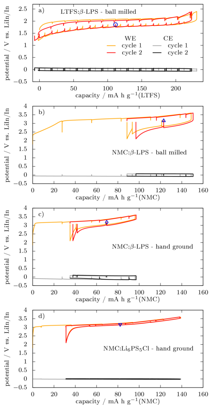
Figure 5: galvanostatic voltage profiles of WE and Li 0.5 In CE for the first 2 cycles in 3 electrodes configuration. WE active material is LTFS (a) or NMC 622 (c-d); WE composites are prepared by high-energy ball milling (a-b) or hand grinding (c-d); electrolyte is β-Li 3 PS 4 (a-c) or Li 6 PS 5 Cl argyrodite (d).
