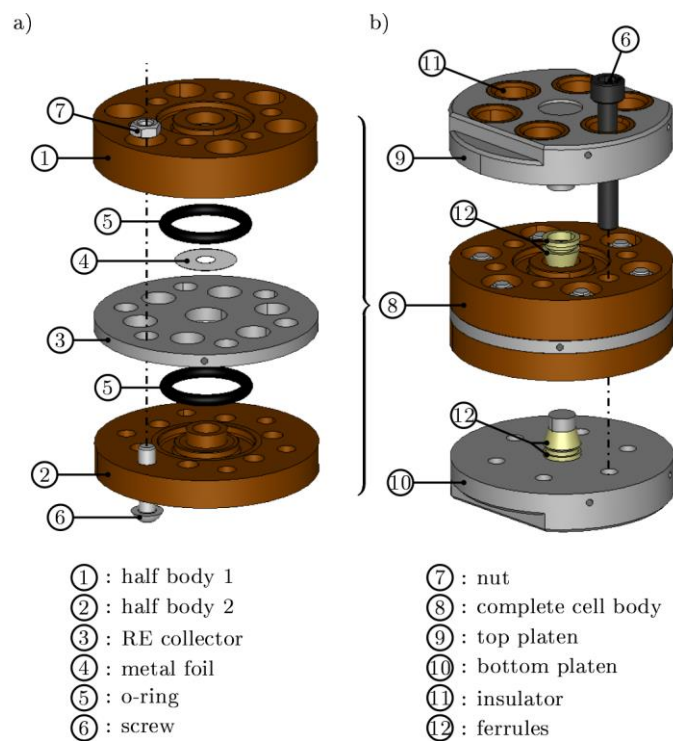
Figure 1: the 3 electrodes cell hardware: a) body; b) complete cell.
