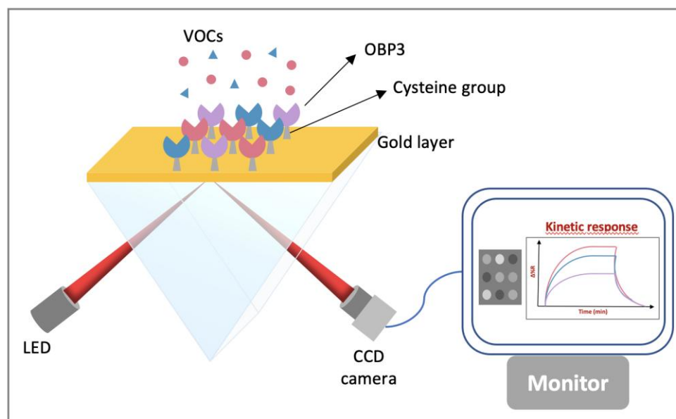
Figure 10. Schematic representation of the SPR-based olfactory biosensor with odorant binding proteins (OBPs) as sensing elements. The three rat OBP3 mutants were immobilized on the gold surface of a prism and their interaction with volatile organic compounds (VOCs) was monitored by SPR imaging.
