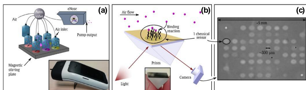
Figure 12. (a) Portable NeOse Pro and the experimental set-up for VOC sampling, (b) working principle and (c) raw image of the prism surface with each spot corresponding to a sensor [188].
