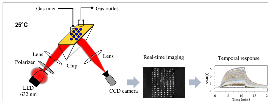
Figure 11. Schematic presentation of the home-made SPR imaging setup.
