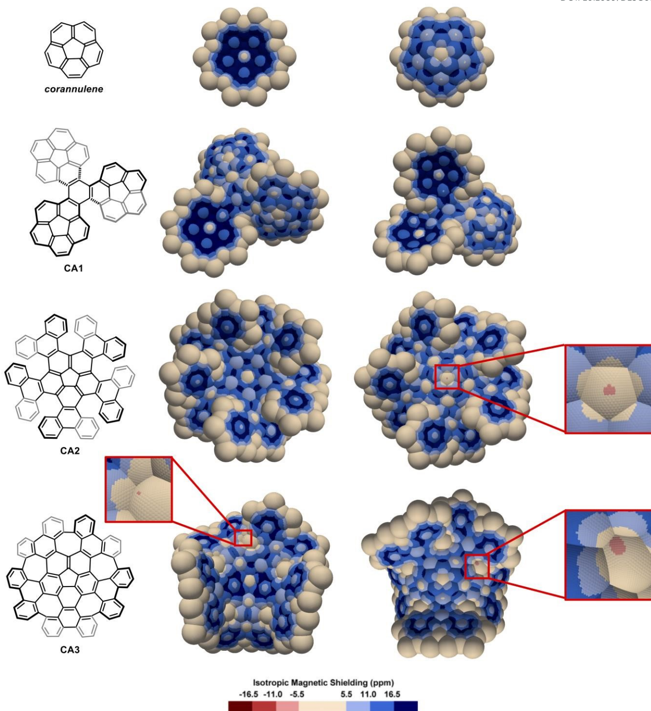
Fig. 6 3D IMS contour maps of corannulene and corannulene-containing nanographenes calculated at the B3LYP-GIAO/6-311++G**//B3LYP-D3BJ/def2SVP level of theory. Both faces of the molecules are shown (horizontal flip for the maps on the right).
