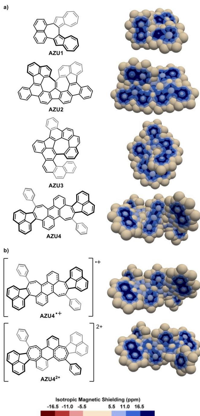
Fig. 7 3D IMS contour maps of azulene-containing hydrocarbons and some corresponding cations calculated at the B3LYP-GIAO/6-311++G**//B3LYP-D3BJ/def2SVP level of theory. a) Neutral molecules. b) Cationic analogues of AZU4 .
