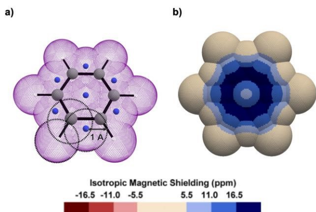
Fig. 1 a) Oblique view of a pseudo-van der Waals surface of Bq (purple colour) generated over benzene by the overlap of 19 spheres of 1 Å radius centred on the C (grey colour), H (white colour), and dummy (artificially introduced at specific barycentres as described in Fig. S1 in the ESI, blue colour) nuclei. b) Top view of the corresponding 3D IMS contour map of benzene calculated at the B3LYP-GIAO/6-311++G**//B3LYP-D3BJ/def2SVP level of theory.
