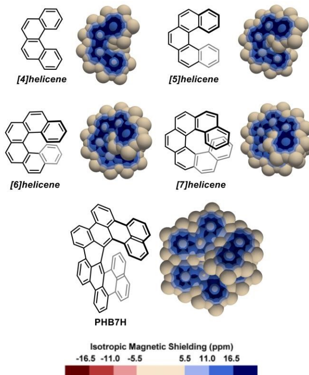
Fig. 2 3D IMS contour maps of [n] helicenes and peri -hexabenzo [7] helicene ( PHB7H ) calculated at the B3LYP-GIAO/6-311++G**//B3LYP-D3BJ/def2SVP level of theory.
