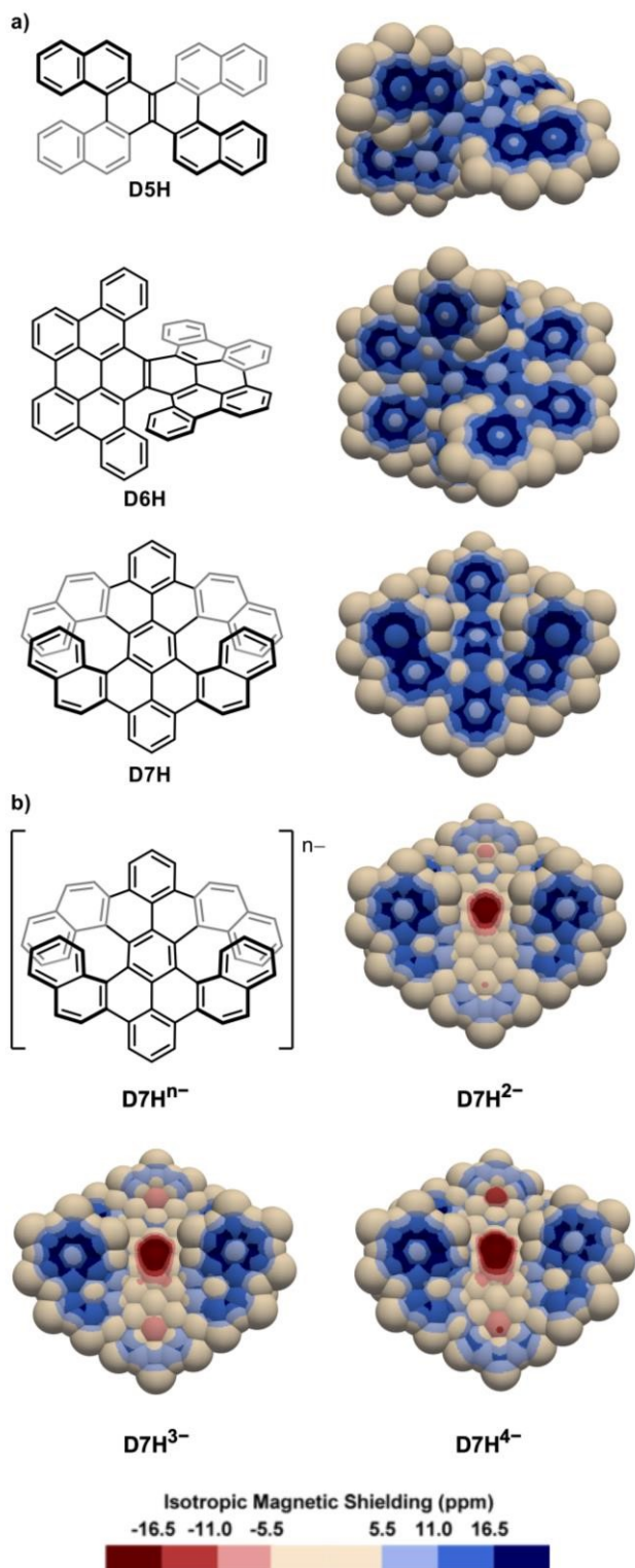
Fig. 4 3D IMS contour maps of double helicenes and some corresponding anions calculated at the B3LYP-GIAO/6-311++G**//B3LYP-D3BJ/def2SVP level of theory. a) Neutral molecules. b) Anionic analogues of D7H .
