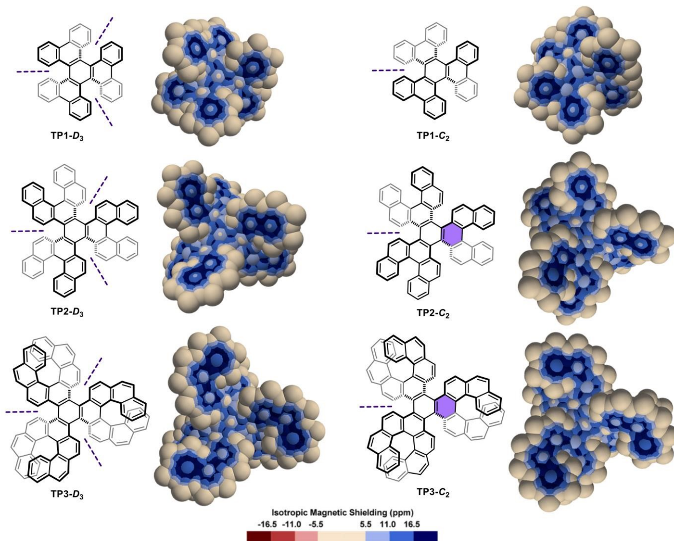
Fig. 3 3D IMS contour maps of triphenylene-centred multi-helicenes, pairs of diastereomers, calculated at the B3LYP-GIAO/6-311++G**//B3LYP-D3BJ/def2SVP level of theory. C_2 symmetry axes are noted with purple dashed lines, and rings with remarkable torsion angles are highlighted with a purple background.
