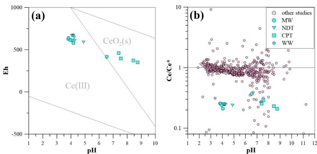
Figure 10 (a): Eh-pH diagram of Ce; (b) relationship between pH and Ce/Ce* (data shown in panel b are the same as used in Fig. 8)
