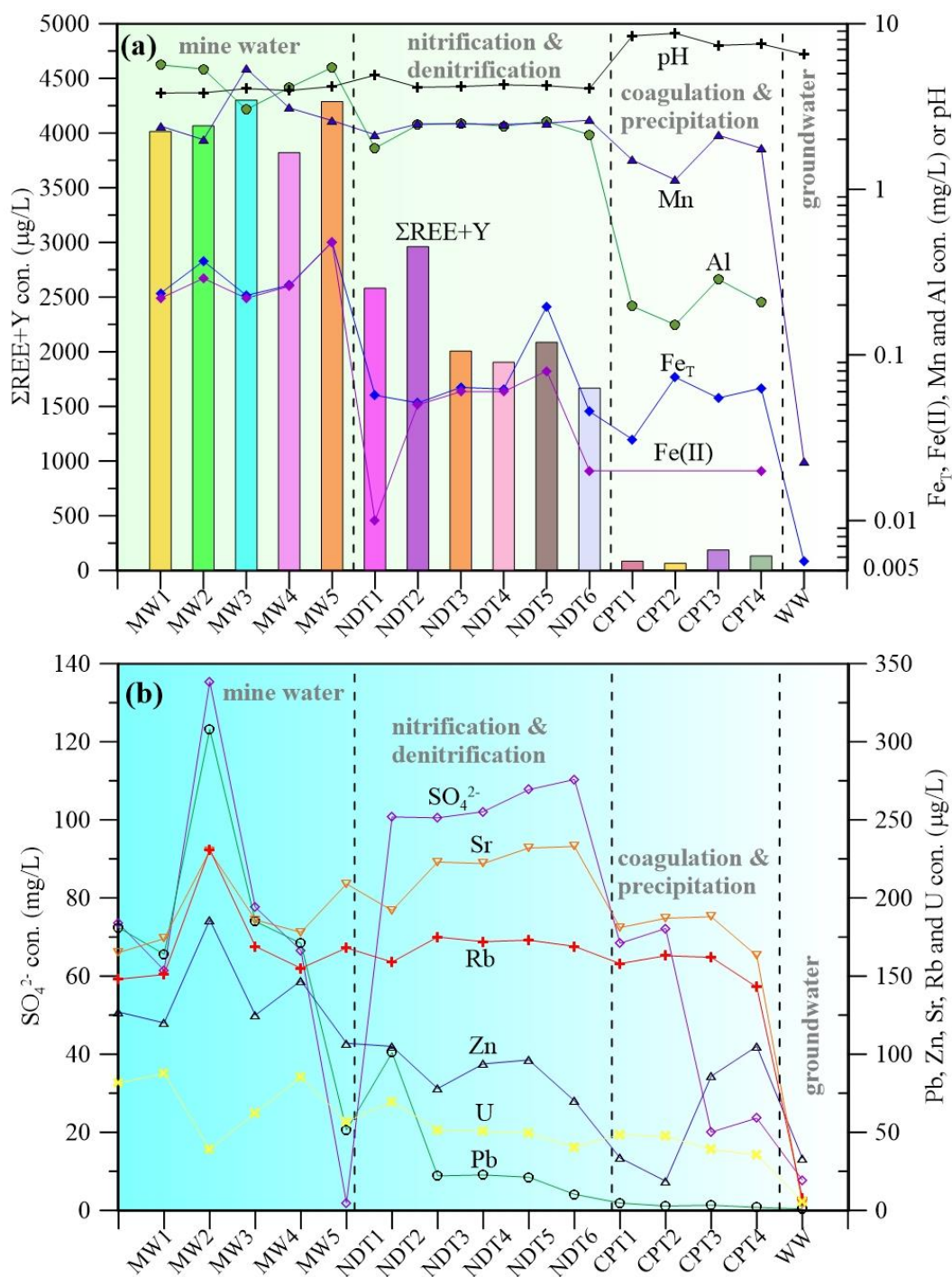
Figure 3 Changes of REE and Y with individual water samples ((a): pH, total REE and Y ( \Sigma REE+Y), total Fe ( Fe_T ), Fe(II), Al and Mn concentrations; (b): SO_4^{2-} , Sr, Rb, Zn, U and Pb concentrations)
