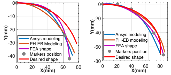
Fig. 9: Shape reconstruction from Mango
