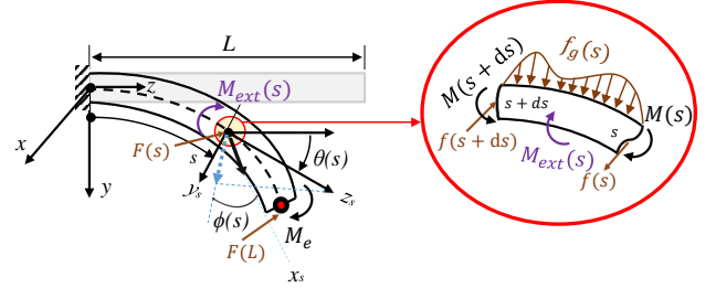
Fig. 2: 3D bending of FEA
