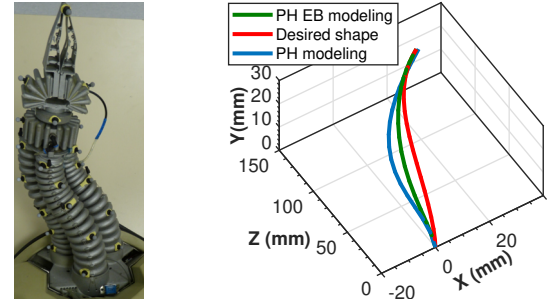
Fig. 10: 3D CBHA Shape in free case
