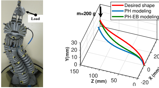
(a) Real soft continuum robot (b) Kinematics reconstruction
