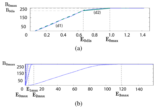
Figure 5: (a) Measured CRF of UI3250-LE, piecewise linearly approximated (( d_1 ) and ( d_2 )), (b) measured CRF for the 4 panoramic regions of the acquired HDROmni image.
