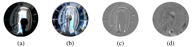
Figure 8: Parking lot 1 of high scene DR. Desired images for pPVS: (a) LDR (b) HDR. Differences between the image at convergence and the desired image for (c) LDR- and (d) HDR-pPVS.
