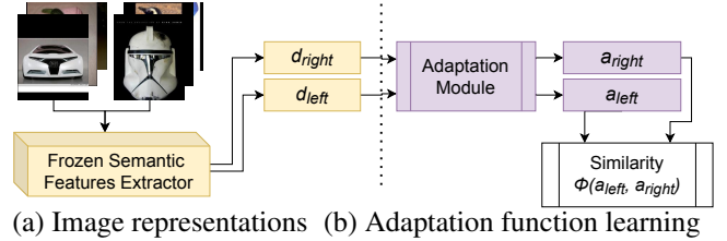
FIGURE 2 – Pipeline to learn an adaptation function able to compute visual similarity from image pairs.
