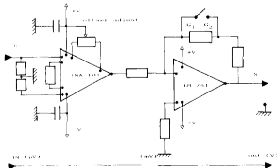
Fig. 3. Two-stage low level thermocouple amplifier.
