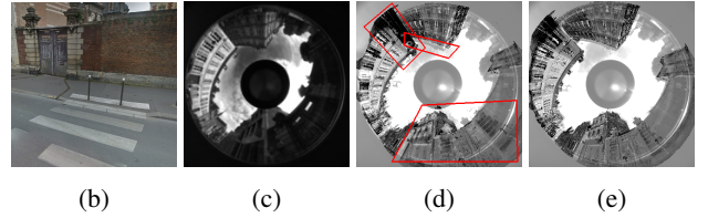
FIGURE 4 – Direct 3D model-based tracking with PGMoT and PoT using 1 frame every N frame(s) : (a) Estimated trajectories on (b) challenging uneven ground where images as (c) are acquired ; (d-e) Superimposition of the last acquired and optimal virtual images ( N = 20 ) : (d) PoT, (e) PGMoT.
