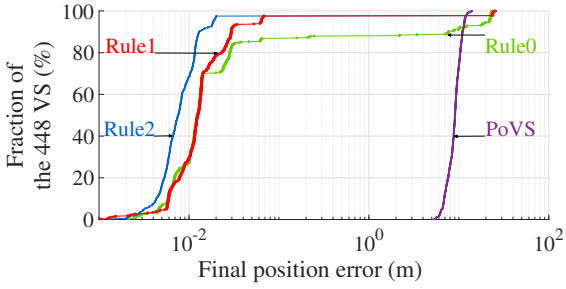
FIGURE 3 – Cumulative distribution of position errors.
