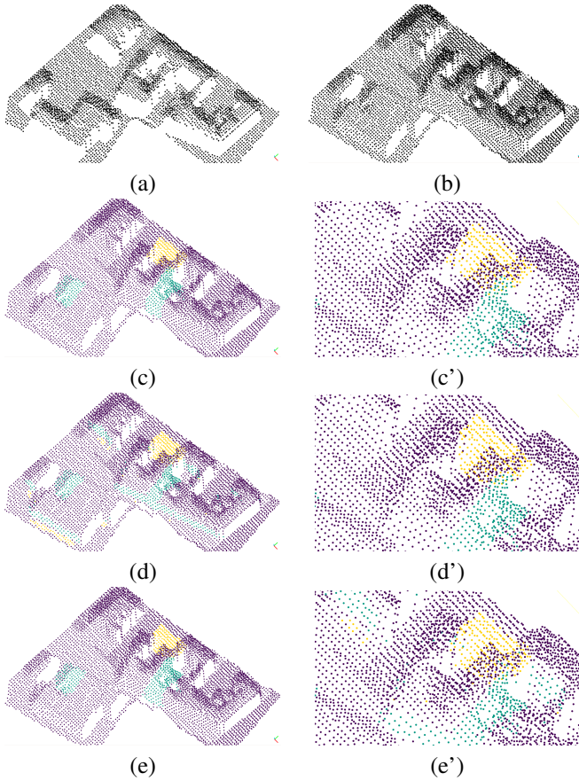
Figure 5: Visual change detection results. (a-b) the two input point clouds ; (c) simulated changes (purple: no change, blue: new construction, yellow: destruction) ; (d) our results; (e) results with [7] method; (') denote close-up views.
