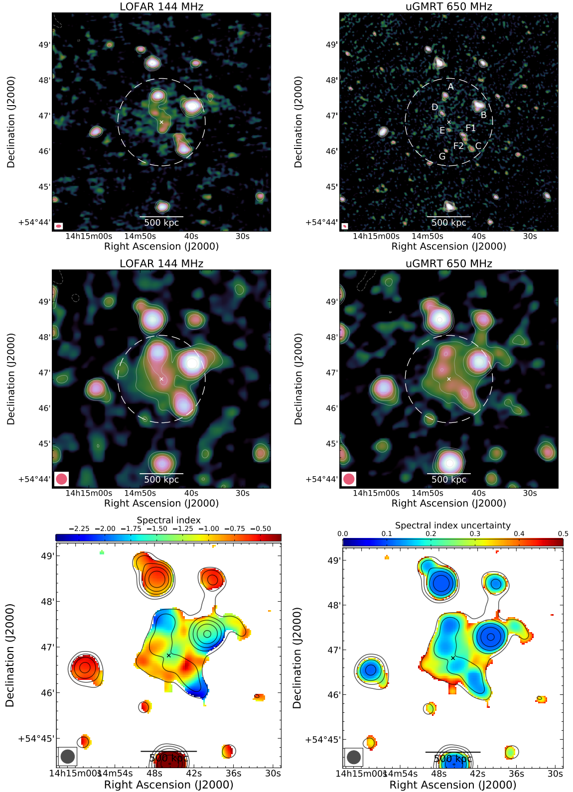
Fig. 4. PSZ2 G099.86+58.45. Top and central rows: full-resolution and 18'' images (weighting='Briggs' and robust=-0.5) at 144 MHz ( left ) and 650 MHz ( right ). White-coloured radio contours are drawn at levels of 2.5\sigma_{\text{rms}} \times [-1, 1, 2, 4, 8, 16, 32] , with \sigma_{\text{rms}} being the noise level at each frequency (see Table 3). The negative contour level is drawn with a dashed white line. We followed Cassano et al. (2019) for the source labelling (their sources 1, 2, and 3 became D, E, and F1+F2, respectively). The dashed white circle in each map shows the R = 0.5R_{\text{SZ},500} region obtained from M_{\text{SZ},500} , with the cross showing the cluster centre. Bottom row: spectral index map between 144 and 650 MHz at 18'' resolution, and correspondent uncertainty map ( left and right panels , respectively). uGMRT radio contours at 650 MHz are drawn in black, at the levels 3\sigma_{\text{rms}} \times [-1, 1, 2, 4, 8, 16, 32] , with \sigma_{\text{rms}} the noise level (see Table 3).
