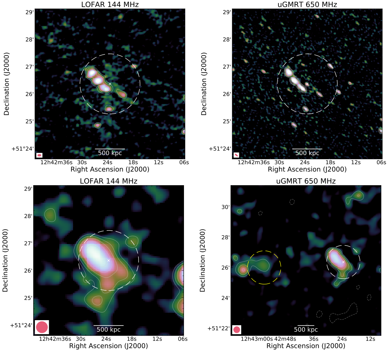
Fig. 5. PSZ2 G126.28+65.62. Top and bottom rows: full-resolution and 25'' images (weighting='Briggs' and robust=-0.5) at 144 MHz ( left ) and 650 MHz ( right ). White-coloured radio contours are drawn at levels of 2.5\sigma_{\text{rms}} \times [-1, 1, 2, 4, 8, 16, 32] , with \sigma_{\text{rms}} being the noise level at each frequency (see Table 3). The negative contour level is drawn with a dashed white line. The dashed white circle in each map shows the R = 0.5R_{\text{SZ},500} region obtained from M_{\text{SZ},500} , with the cross showing the cluster centre. The dashed yellow circle in the bottom right panel shows the position of the mock radio halo.
