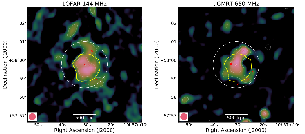
Fig. A.8. PSZ2 G147.88+53.24. 22''-resolution compact source-subtracted LOFAR and uGMRT images at 144 MHz (left) and 650 MHz(right). White-coloured radio contours at the same resolution are drawn at levels of 2.5\sigma_{\text{rms}} \times [-1, 1, 2, 4, 8, 16, 32] , with \sigma_{\text{rms},144} = 140 \mu\text{Jy beam}^{-1} and \sigma_{\text{rms},650} = 35 \mu\text{Jy beam}^{-1} the maps noise. The negative contour level is drawn with a dashed white line. The dashed white circle in each map shows the R = 0.5R_{\text{SZ},500} region obtained from M_{\text{SZ},500} , with the white cross showing the cluster centre. The positions of the subtracted sources in the cluster region are highlighted with red crosses. The yellow polygon represents the area where the flux densities were measured.
