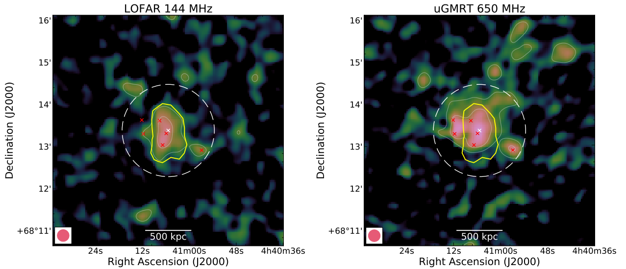
Fig. A.6. PS22 G141.77+14.19. 17''-resolution compact source-subtracted LOFAR and uGMRT images at 144 MHz (left) and 650 MHz (right). White-coloured radio contours at the same resolution are drawn at levels of 2.5\sigma_{\text{rms}} \times [-1, 1, 2, 4, 8, 16, 32] , with \sigma_{\text{rms},144} = 165 \mu\text{Jy beam}^{-1} and \sigma_{\text{rms},650} = 20 \mu\text{Jy beam}^{-1} the maps noise. The negative contour level is drawn with a dashed white line. The dashed white circle in each map shows the R = 0.5R_{\text{SZ},500} region obtained from M_{\text{SZ},500} , with the white cross showing the cluster centre. The positions of the subtracted sources in the cluster region are highlighted with red crosses. The yellow polygon represents the area where the flux densities were measured.
