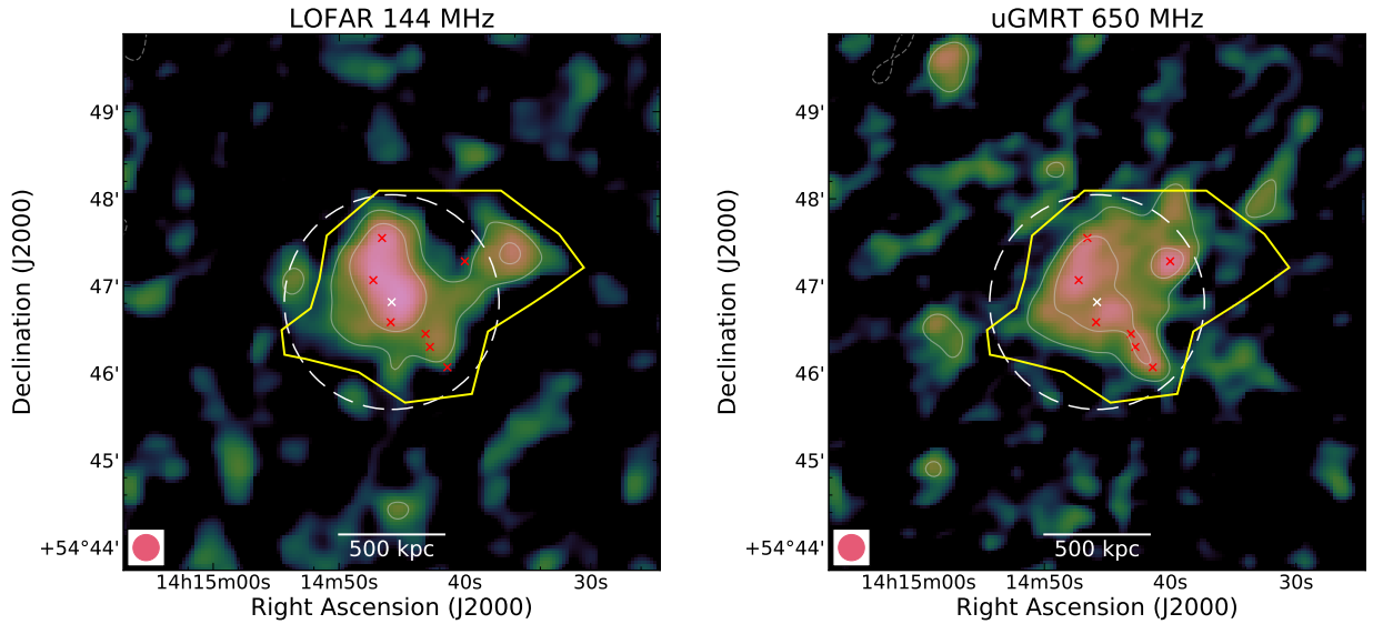
Fig. A.4. PSZ2 G099.86+58.45 18'' -resolution compact source-subtracted LOFAR and uGMRT images at 144 MHz (left) and 650 MHz(right). White-coloured radio contours at the same resolution are drawn at levels of 2.5\sigma_{\text{rms}} \times [-1, 1, 2, 4, 8, 16, 32] , with \sigma_{\text{rms},144} = 140 \mu\text{Jy beam}^{-1} and \sigma_{\text{rms},650} = 32 \mu\text{Jy beam}^{-1} the maps noise. The negative contour level is drawn with a dashed white line. The dashed white circle in each map shows the R = 0.5R_{\text{SZ},500} region obtained from M_{\text{SZ},500} , with the white cross showing the cluster centre. The positions of the subtracted sources in the cluster region are highlighted with red crosses. The yellow polygon represents the area where the flux densities were measured.
