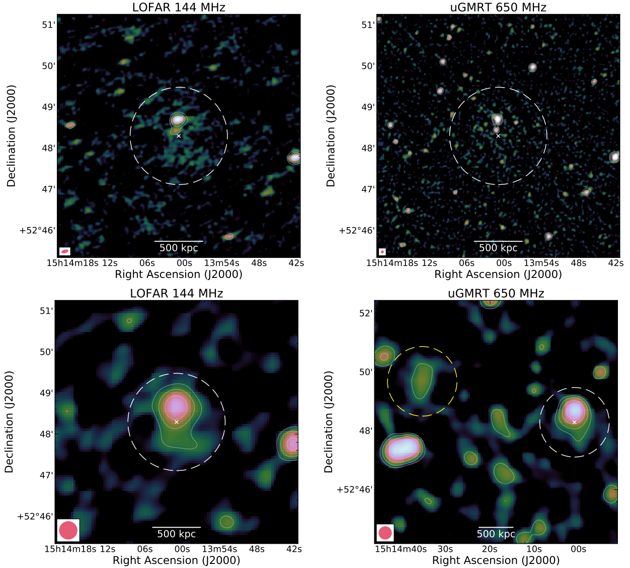
Fig. 1. PSZ2 G086.93+53.18. Top and bottom rows: full-resolution and 26'' images (weighting='Briggs' and robust=-0.5) at 144 MHz (left) and 650 MHz (right). White-coloured radio contours are drawn at levels of 2.5\sigma_{\text{rms}} \times [-1, 1, 2, 4, 8, 16, 32] , with \sigma_{\text{rms}} being the noise level at each frequency (see Table 3). The negative contour level is drawn with a dashed white line. The dashed white circle in each map shows the R = 0.5R_{SZ,500} region obtained from M_{SZ,500} , with the cross showing the cluster centre. The dashed yellow circle in the bottom right panel shows the position of the mock radio halo.
