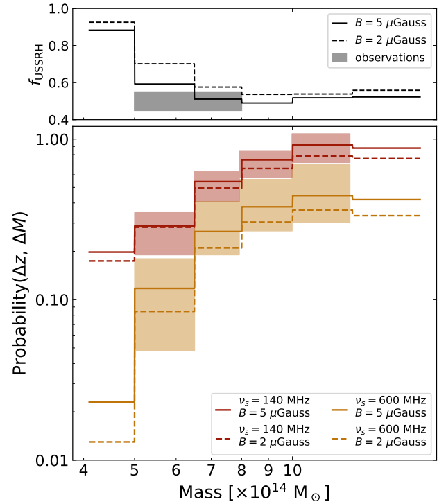
Fig. 12. Probability of forming radio halos with \nu_s > 140 and \nu_s > 600 MHz (red and yellow lines, respectively) as a function of the cluster virial mass in the redshift range 0.6–0.7. Magnetic fields of B = 5 \mu\text{Gauss} and B = 2 \mu\text{Gauss} are assumed (solid and dashed lines, respectively). The shadowed regions represent the 1\sigma uncertainty derived through Monte Carlo calculations. Top panel: expected fraction of USSRH visible at 144 MHz with steepening frequency \nu_s < 600 MHz as a function of the cluster virial mass, assuming B = 5 \mu\text{Gauss} and B = 2 \mu\text{Gauss} (solid and dashed lines, respectively). The shadowed area indicates the observed fraction of USSRH in our sample.
