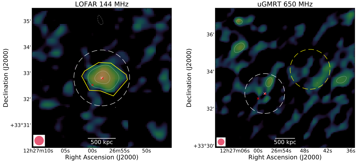
Fig. A.9. PS22 G160.83+81.66. 22''-resolution compact source-subtracted LOFAR and uGMRT images at 144 MHz (left) and 650 MHz (right). White-coloured radio contours at the same resolution are drawn at levels of 2.5\sigma_{\text{rms}} \times [-1, 1, 2, 4, 8, 16, 32] , with \sigma_{\text{rms}} the noise map (see Table 3). The negative contour level is drawn with a dashed white line. The dashed white circle in each map shows the R = 0.5R_{\text{SZ},500} region obtained from M_{\text{SZ},500} , with the white cross showing the cluster centre, while the dashed yellow circle shows the position of the injected mock halo. The positions of the subtracted sources in the cluster region are highlighted with red crosses. The yellow polygon represents the area where the flux densities were measured.
