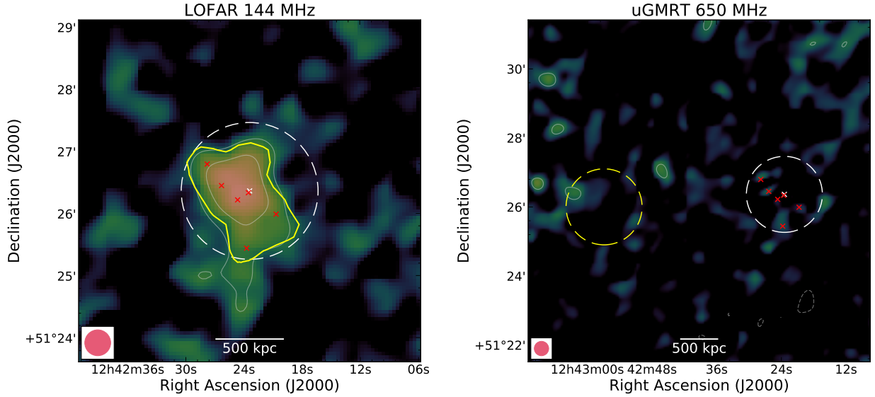
Fig. A.5. PS22 G126.28+65.62. 25''-resolution compact source-subtracted LOFAR and uGMRT images at 144 MHz (left) and 650 MHz (right). White-coloured radio contours at the same resolution are drawn at levels of 2.5\sigma_{\text{rms}} \times [-1, 1, 2, 4, 8, 16, 32] , with \sigma_{\text{rms},144} = 130 \mu\text{Jy beam}^{-1} and \sigma_{\text{rms},650} = 80 \mu\text{Jy beam}^{-1} the maps noise. The negative contour level is drawn with a dashed white line. The dashed white circle in each map shows the R = 0.5R_{\text{SZ},500} region obtained from M_{\text{SZ},500} , with the white cross showing the cluster centre, while the dashed yellow circle shows the position of the injected mock halo. The positions of the subtracted sources in the cluster region are highlighted with red crosses. The yellow polygon represents the area where the flux densities were measured.
