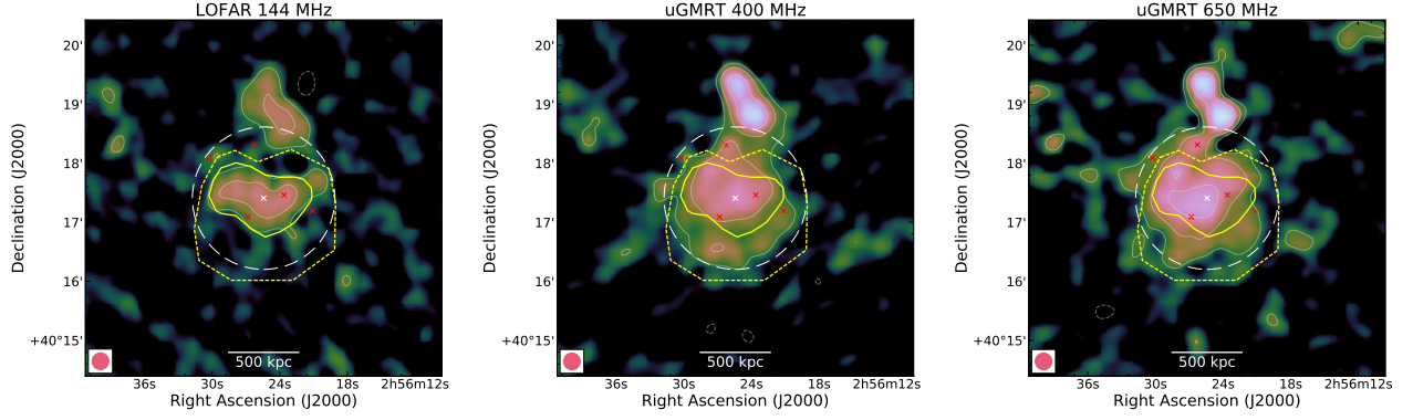
Fig. A.7. PLCK G147.3–16.6. 17''-resolution compact source-subtracted LOFAR and uGMRT images at 144 MHz (left), 400 MHz (middle) and 650 MHz(right). White-coloured radio contours at the same resolution are drawn at levels of 2.5\sigma_{\text{rms}} \times [-1, 1, 2, 4, 8, 16, 32] , with \sigma_{\text{rms},144} = 300 \mu\text{Jy beam}^{-1} , \sigma_{\text{rms},400} = 61 \mu\text{Jy beam}^{-1} and \sigma_{\text{rms},650} = 25 \mu\text{Jy beam}^{-1} the maps noise. The negative contour level is drawn with a dashed white line. The dashed white circle in each map shows the R = 0.5R_{\text{SZ},500} region obtained from M_{\text{SZ},500} , with the white cross showing the cluster centre. The positions of the subtracted sources in the cluster region are highlighted with red crosses. The yellow solid and dashed polygons represent the area where the flux densities were measured.
