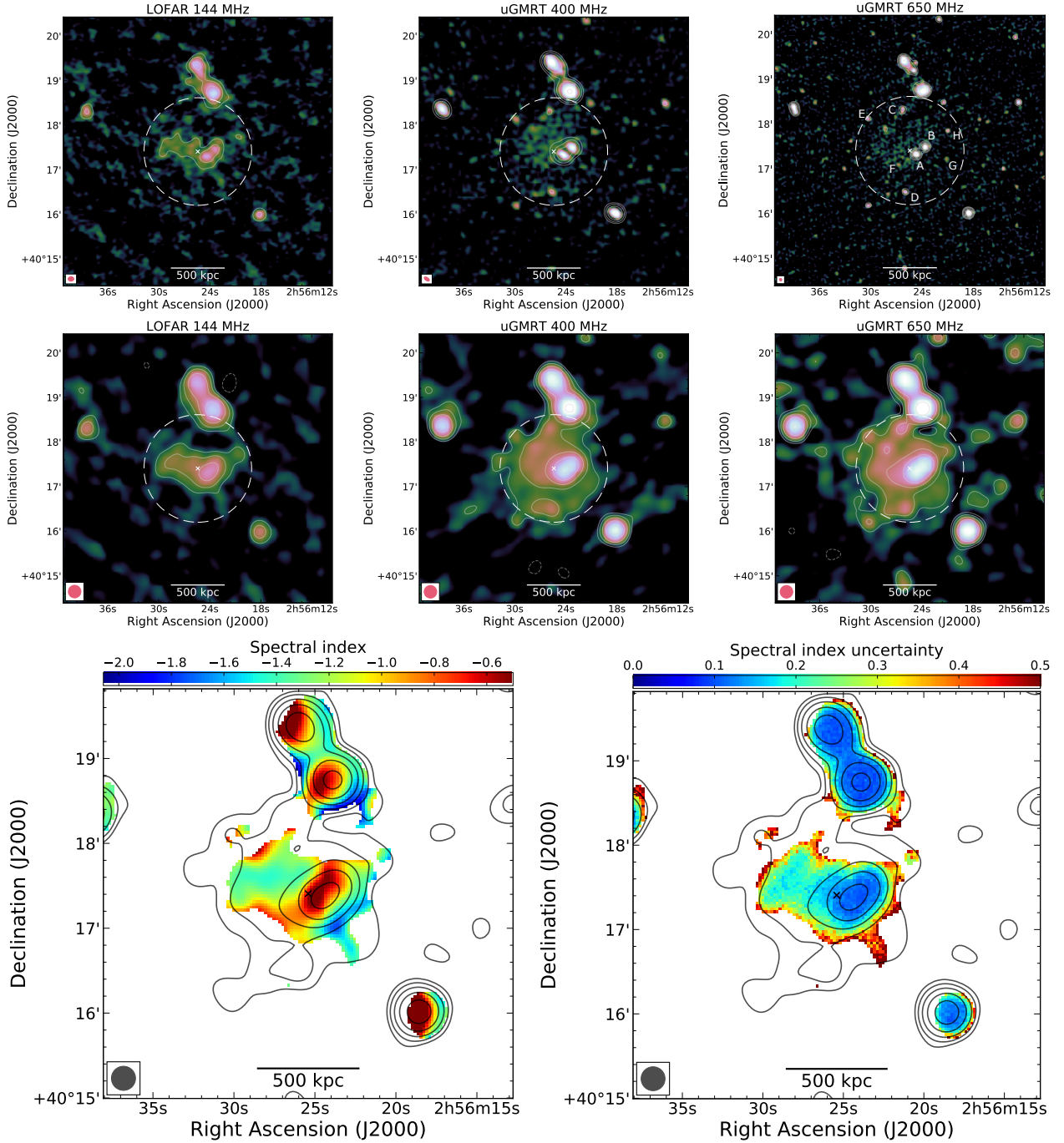
Fig. 7. PLCK G147.3–16.6. Top and central rows: full-resolution and 17'' images (weighting='Briggs' and robust=-0.5) at 144 MHz ( left ), 400 MHz ( middle ) and 650 MHz ( right ). Radio contours are drawn in white at levels of 2.5\sigma_{\text{rms}} \times [-1, 1, 2, 4, 8, 16, 32] , with \sigma_{\text{rms}} being the noise level at each frequency (see Table 3). The negative contour level is drawn with a dashed white line. We followed van Weeren et al. (2014) for the source labelling. The dashed white circle in each map shows the R = 0.5R_{\text{SZ},500} region, obtained from M_{\text{SZ},500} , with the cross showing the cluster centre. Bottom row: spectral index map at 400 MHz (see Sect. 3.1), at 17'' resolution, and correspondent uncertainty map ( left and right panels , respectively). uGMRT radio contours at 650 MHz are drawn in black, at the levels 3\sigma_{\text{rms}} \times [-1, 1, 2, 4, 8, 16, 32] , with \sigma_{\text{rms}} the noise level (see Table 3).
