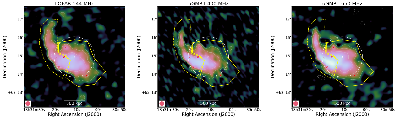
Fig. A.3. PSZ2 G091.83+26.11. 14'' -resolution compact source-subtracted LOFAR and uGMRT images at 144 MHz (left), 400 MHz (middle) and 650 MHz(right). White-coloured radio contours at the same resolution are drawn at levels of 2.5\sigma_{\text{rms}} \times [-1, 1, 2, 4, 8, 16, 32] , with \sigma_{\text{rms},144} = 180 \mu\text{Jy beam}^{-1} , \sigma_{\text{rms},400} = 90 \mu\text{Jy beam}^{-1} and \sigma_{\text{rms},650} = 38 \mu\text{Jy beam}^{-1} the maps noise. The negative contour level is drawn with a dashed white line. The dashed white circle in each map shows the R = 0.5R_{\text{SZ},500} region obtained from M_{\text{SZ},500} , with the white cross showing the cluster centre. The positions of the subtracted sources in the cluster region are highlighted with red crosses. The yellow polygons represent the area where the flux densities were measured for the halo (solid) and the relic (dashed).
