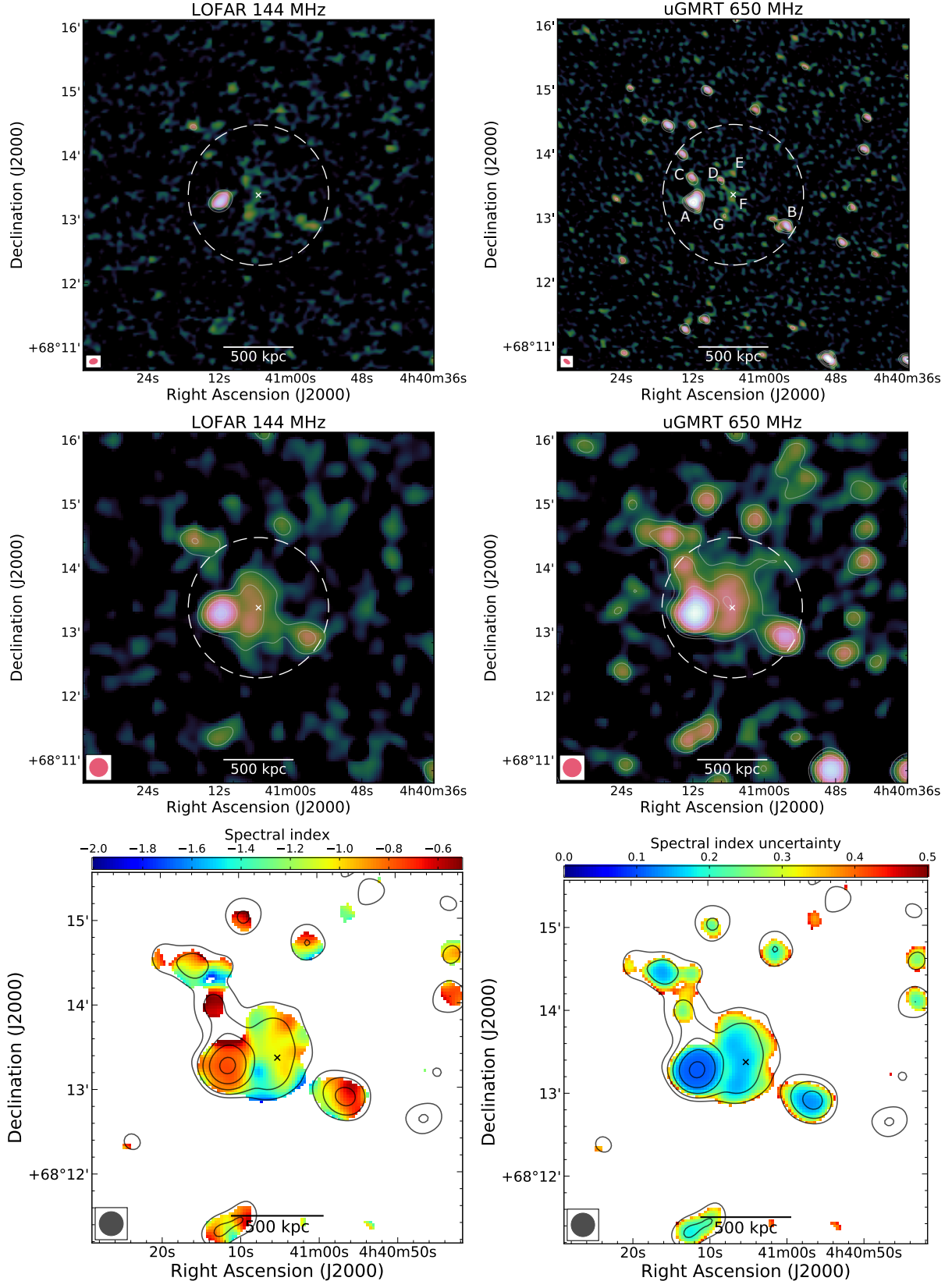
Fig. 6. PSZ2 G141.77+14.19 . Top and central rows: full-resolution and 17'' images (weighting='Briggs' and robust=-0.5) at 144 MHz ( left ) and 650 MHz ( right ). White-coloured radio contours are drawn at levels of 2.5\sigma_{\text{rms}} \times [-1, 1, 2, 4, 8, 16, 32] , with \sigma_{\text{rms}} being the noise level at each frequency (see Table 3). The negative contour level is drawn with a dashed white line. The dashed white circle in each map shows the R = 0.5R_{\text{SZ},500} region obtained from M_{\text{SZ},500} , with the cross showing the cluster centre. Bottom row: spectral index map between 144 and 650 MHz at 17'' resolution, and correspondent uncertainty map ( left and right panels , respectively). uGMRT radio contours at 650 MHz are drawn in black, at the levels 3\sigma_{\text{rms}} \times [-1, 1, 2, 4, 8, 16, 32] , with \sigma_{\text{rms}} being the noise level (see Table 3).
