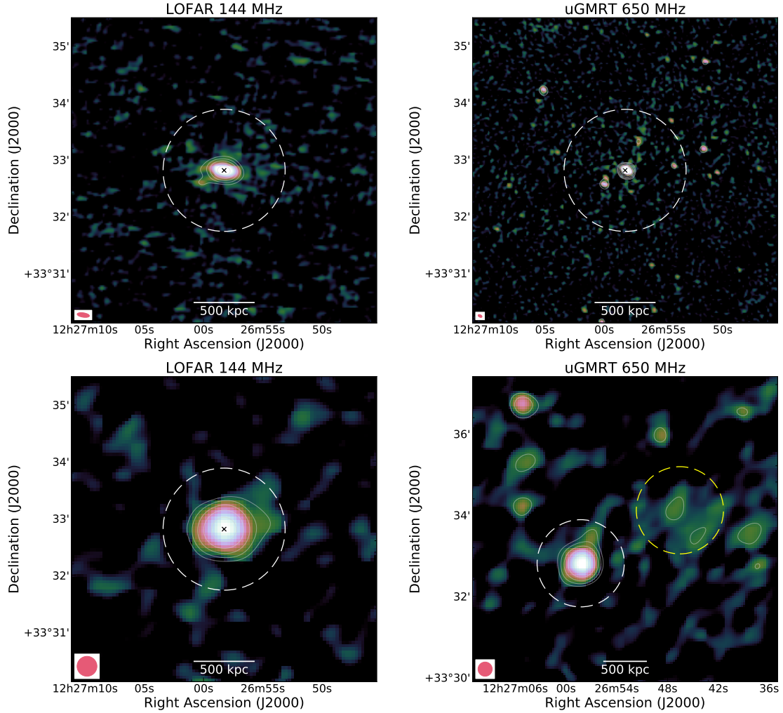
Fig. 9. PSZ2 G160.83+81.66. Top and bottom rows: full-resolution and 21'' images (weighting='Briggs' and robust=-0.5) at 144 MHz ( left ) and 650 MHz ( right ). White-coloured radio contours are drawn at levels of 2.5\sigma_{\text{rms}} \times [-1, 1, 2, 4, 8, 16, 32] , with \sigma_{\text{rms}} being the noise level at each frequency (see Table 3). The negative contour level is drawn with a dashed white line. The dashed white circle in each map shows the R = 0.5R_{\text{SZ},500} region, obtained from M_{\text{SZ},500} , with the cross showing the cluster centre. The dashed yellow circle in the bottom right panel shows the position of the mock radio halo.
