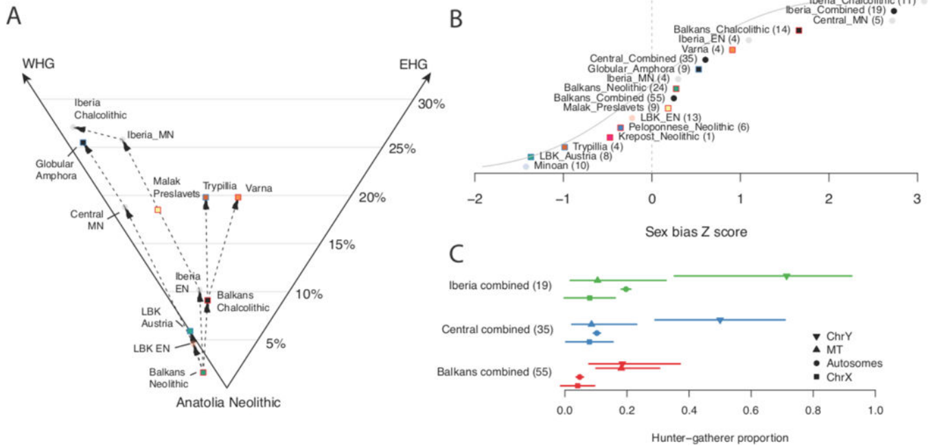
Figure 3. Structure and change in NW Anatolian Neolithic-related populations A: Populations modeled as a mixture of NW Anatolia Neolithic, WHG, and EHG. Dashed lines show temporal relationships between populations from the same geographic region. Percentages indicate proportion of WHG+EHG ancestry. Standard errors range from 0.7-6.0% (Supplementary Table S3.2.2). B: Z-scores for the difference in hunter-gatherer-related ancestry on the autosomes compared to the X chromosome when populations are modeled as a mixture of NW Anatolia Neolithic and WHG (N=126 individuals, group sizes in parentheses). Positive values indicate more hunter-gatherer-related ancestry on the autosomes and thus male-biased hunter-gatherer ancestry. “Combined” populations merge all individuals from different times from a geographic area. C: Hunter-gatherer-related ancestry proportions on the autosomes, X chromosome, mitochondrial DNA (i.e. mt haplogroup U), and the Y chromosome (i.e. Y chromosome haplogroups I2, R1 and C1). Points show qpAdm (autosomes and X chromosome) or maximum likelihood (MT and Y chromosome) estimates and bars show approximate 95% confidence intervals (N=109 individuals, group sizes in parentheses).
