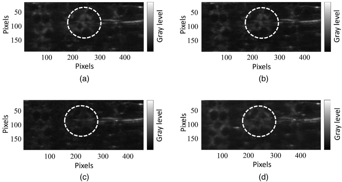
FIGURE 9 Maximum intensity projection based on the DCE-US recordings of UCAs passing through the porous phantom. The white contour indicates the region of interest where the TICs were extracted. (a) Antibubbles. (b) Reference bubbles. (c) SonoVue™ with a peak concentration as in the static measurement. (d) SonoVue™ with a peak concentration 30 times higher than in the static measurement
