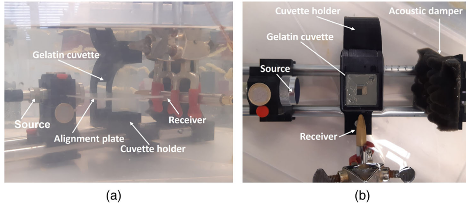
FIGURE 3 The setup for scatter measurements: (a) side view and (b) top view
