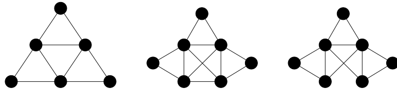
Figure 10: The Hajós graph, the rising sun and the X_1 graph.
