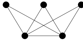
Figure 6: The crown is not a biclique graph but has every P_3 in a diamond.
