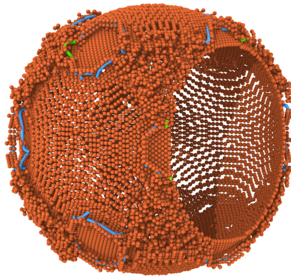
Fig. 5 Relaxed atomic structure of a 15 nm diameter iron cavity with an applied pressure of 10.2 GPa. Only Fe atoms (red spheres) with a coordination number lower than 8 are shown for a better visualization of the cavity external and internal surfaces. A part of the cavity is also cut for sake of clarity. Blue and green tubular lines represent dislocations with \langle 100 \rangle and 1/2\langle 111 \rangle Burgers vectors, respectively, as determined using the dislocation extraction algorithm (Stukowski et al. 2012) implemented in OVITO (Stukowski 2010)
